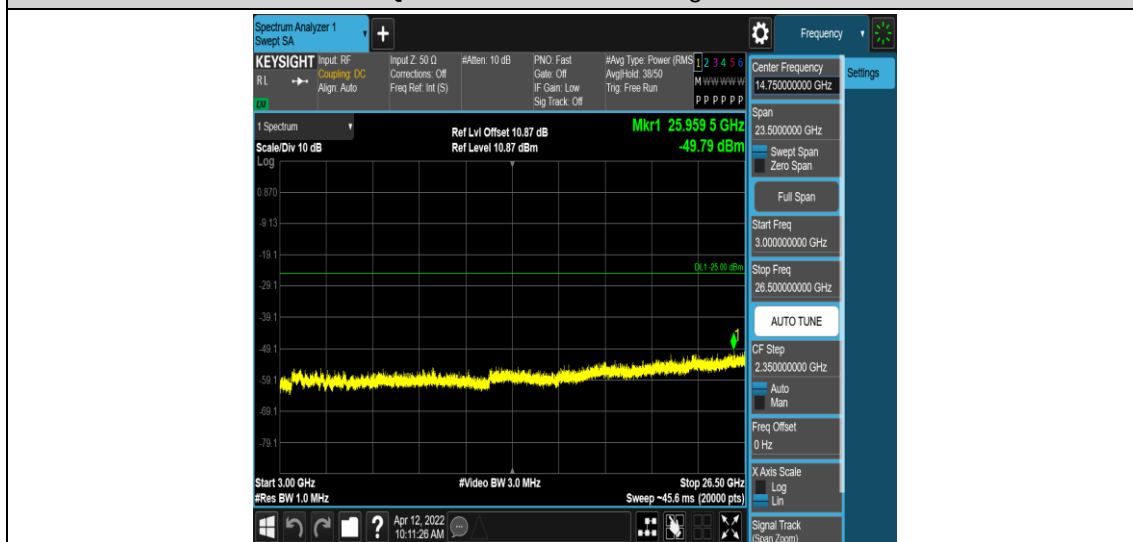
Band7-5MHz-QPSK-21100-1RB#0-Range5:3000~26500MHz
