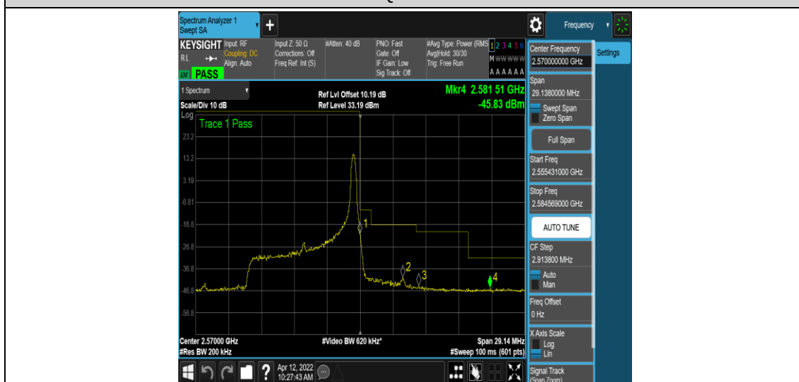
Band7-10MHz-QPSK-21400-1RB#49
