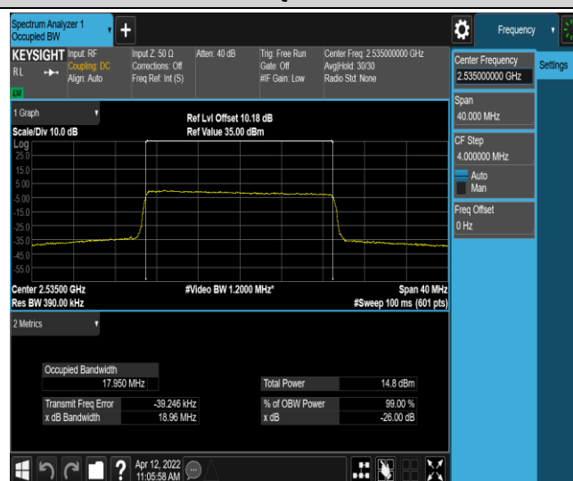
Band7-20MHz-16QAM-21100-100RB#0
