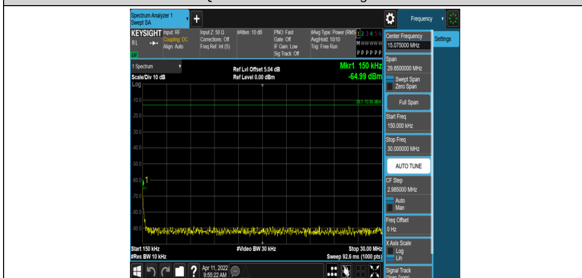
Band5-1.4MHz-QPSK-20643-1RB#0-Range2:0.15~30MHz
