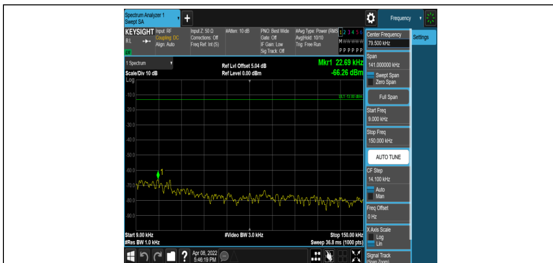
Band4-10MHz-QPSK-20350-1RB#0-Range1:0.009~0.15MHz
