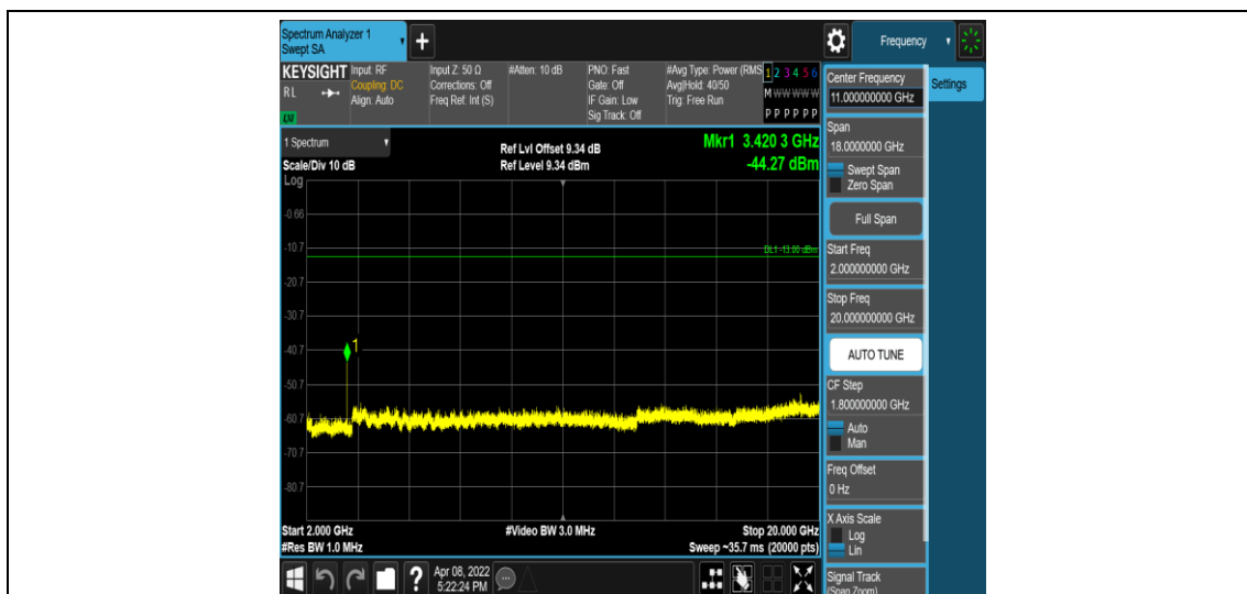
Band4-5MHz-QPSK-19975-1RB#0-Range5:2000~20000MHz
