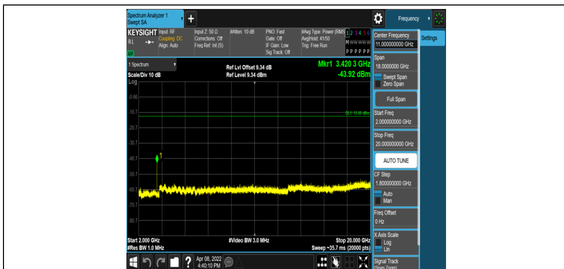
Band4-1.4MHz-16QAM-19957-1RB#0-Range5:2000~20000MHz
