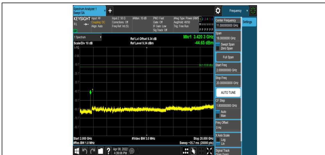
Band4-1.4MHz-QPSK-19957-1RB#0-Range5:2000~20000MHz
