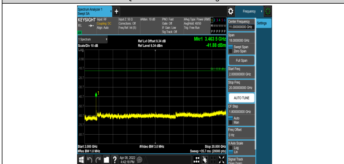
Band4-1.4MHz-16QAM-20175-1RB#0-Range5:2000~20000MHz
