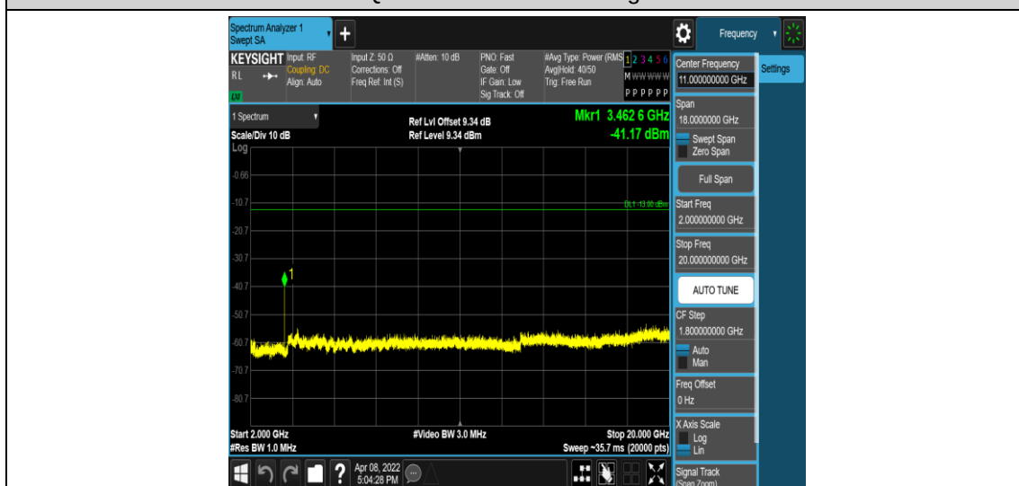
Band4-3MHz-16QAM-20175-1RB#0-Range5:2000~20000MHz
