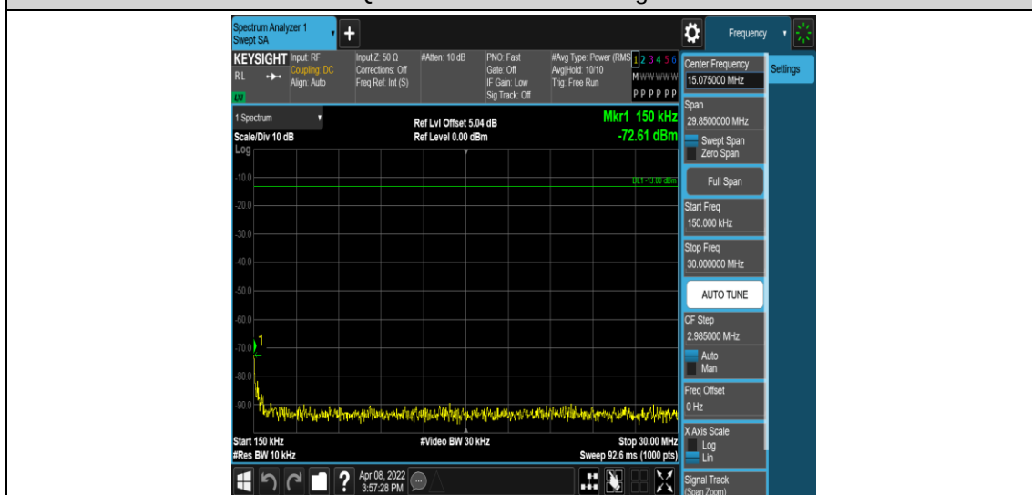
Band2-15MHz-QPSK-18900-1RB#0-Range2:0.15~30MHz
