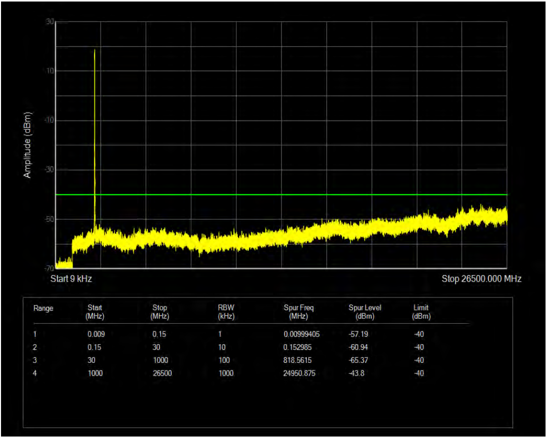
Band30 QAM16 BW=5MHz Channel=27685 RB Size=25 Position=#0
