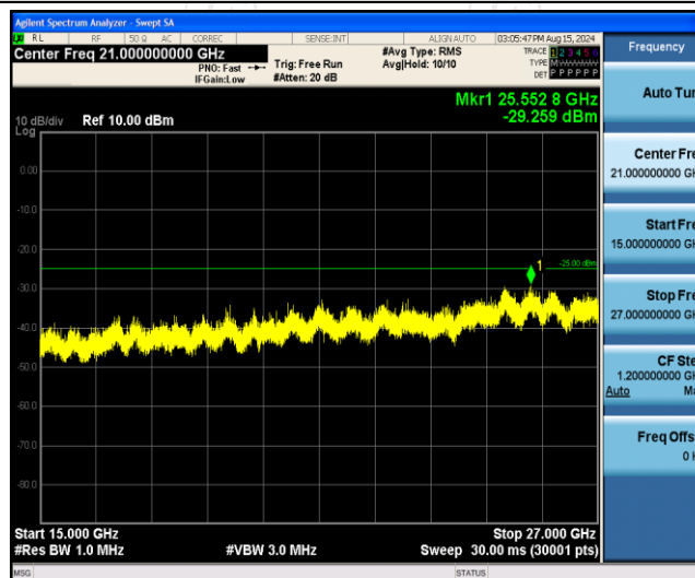
Band7-15MHz-16QAM-21375-1RB#0-Range3:15000~27000MHz
