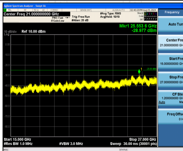
Band7-5MHz-16QAM-21425-1RB#0-Range3:15000~27000MHz
