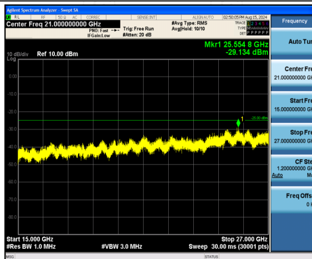
Band7-10MHz-16QAM-20800-1RB#0-Range3:15000~27000MHz
