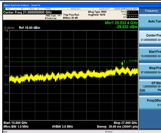
Band7-15MHz-16QAM-21100-1RB#0-Range3:15000~27000MHz
