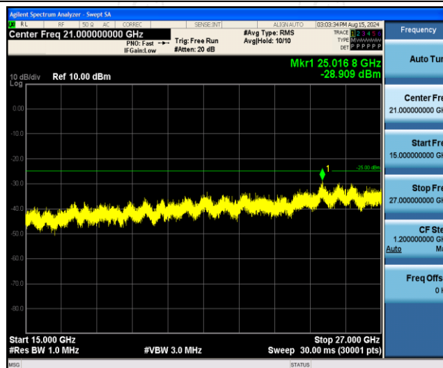
Band7-15MHz-QPSK-21100-1RB#0-Range3:15000~27000MHz
