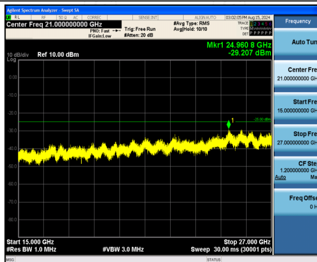
Band7-15MHz-QPSK-20825-1RB#0-Range3:15000~27000MHz
