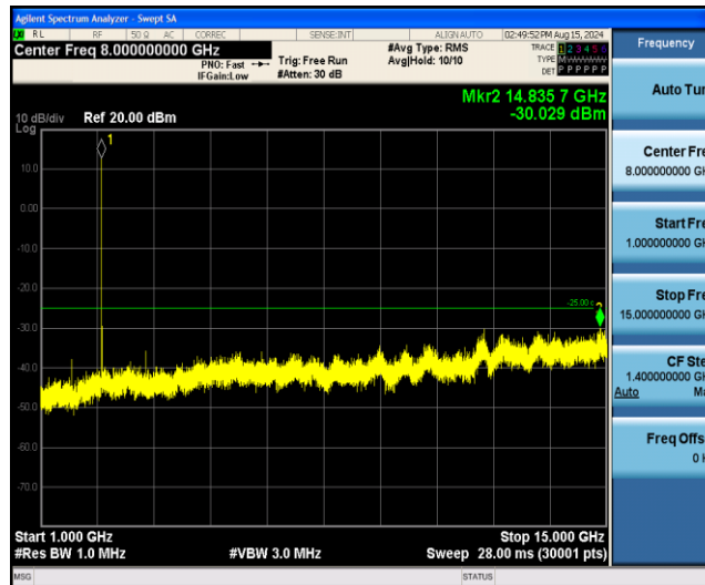
Band7-10MHz-16QAM-20800-1RB#0-Range2:1000~15000MHz
