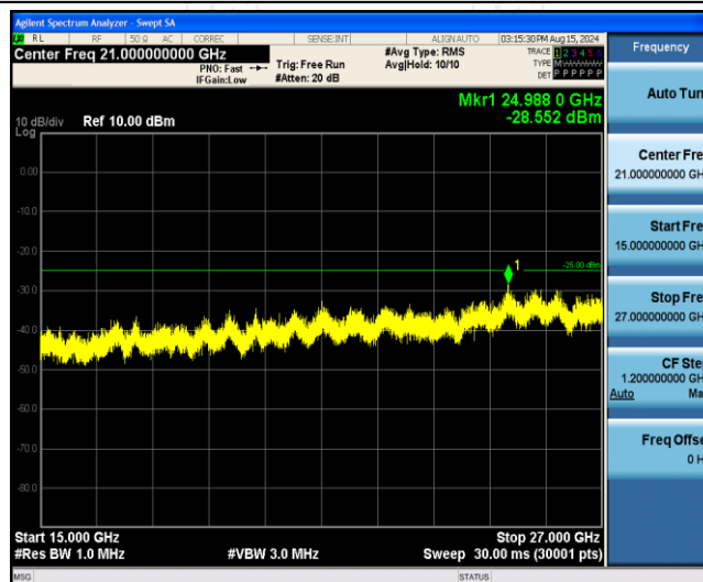
Band7-20MHz-16QAM-20850-1RB#0-Range3:15000~27000MHz
