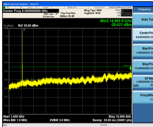
Band7-15MHz-QPSK-21100-1RB#0-Range2:1000~15000MHz
