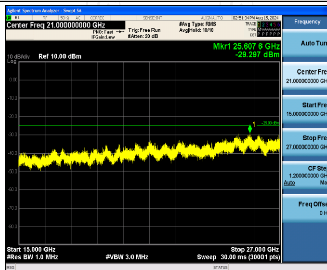
Band7-10MHz-16QAM-21100-1RB#0-Range3:15000~27000MHz
