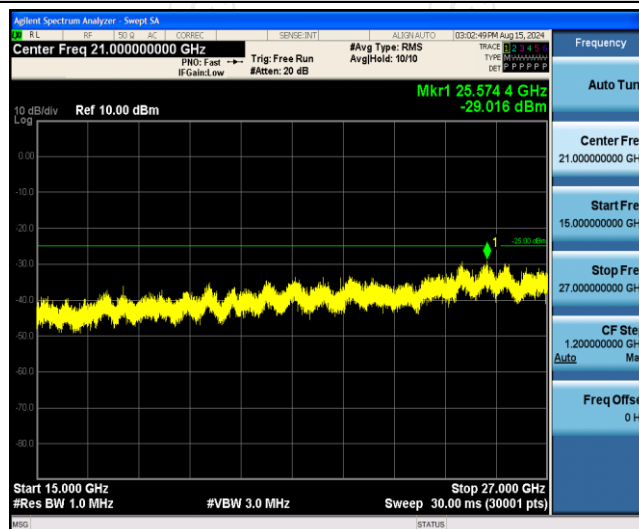
Band7-15MHz-16QAM-20825-1RB#0-Range3:15000~27000MHz
