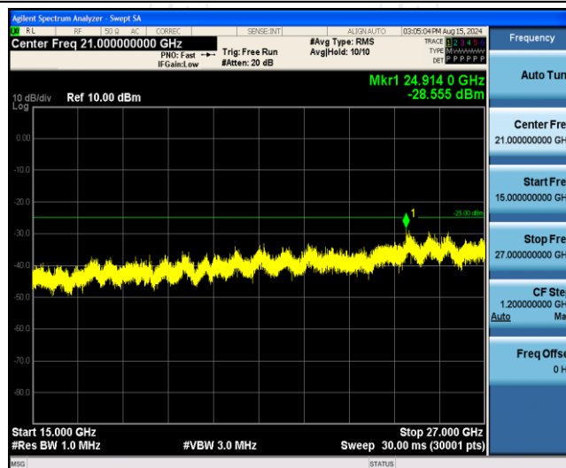
Band7-15MHz-QPSK-21375-1RB#0-Range3:15000~27000MHz
