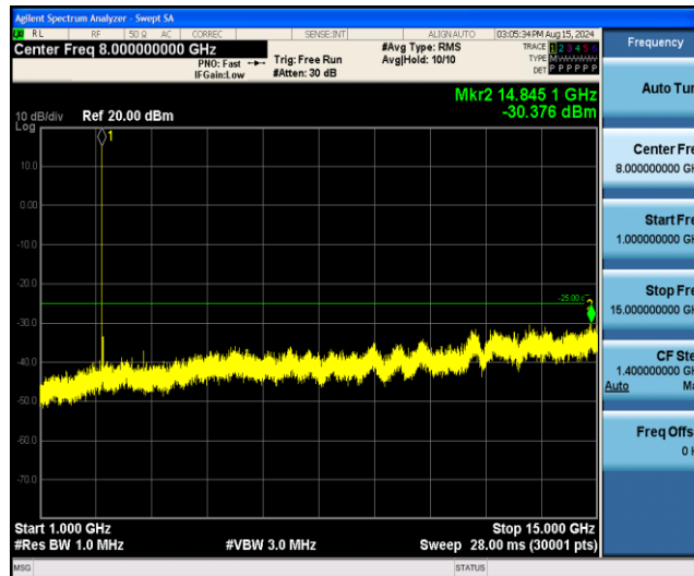
Band7-15MHz-16QAM-21375-1RB#0-Range2:1000~15000MHz
