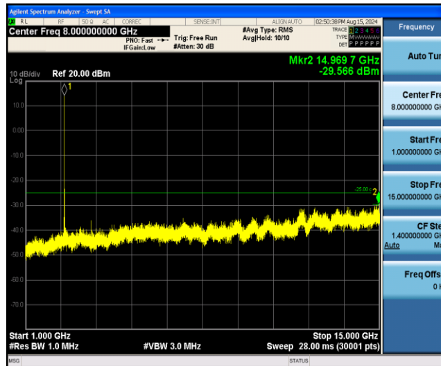
Band7-10MHz-QPSK-21100-1RB#0-Range2:1000~15000MHz
