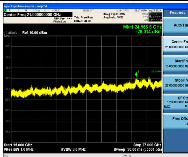
Band7-20MHz-16QAM-21100-1RB#0-Range3:15000~27000MHz
