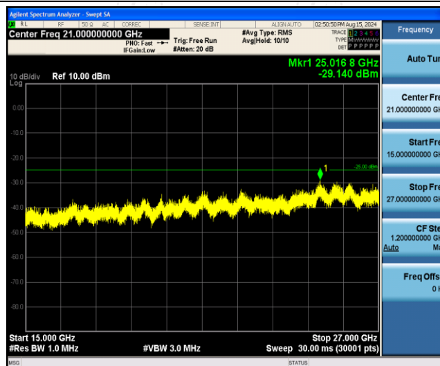
Band7-10MHz-QPSK-21100-1RB#0-Range3:15000~27000MHz
