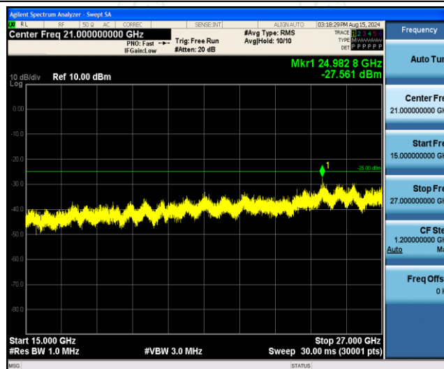
Band7-20MHz-16QAM-21350-1RB#0-Range3:15000~27000MHz
