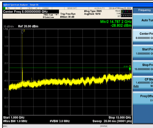
Band7-20MHz-16QAM-21100-1RB#0-Range2:1000~15000MHz
