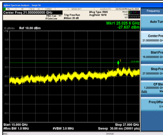
Band7-10MHz-16QAM-21400-1RB#0-Range3:15000~27000MHz
