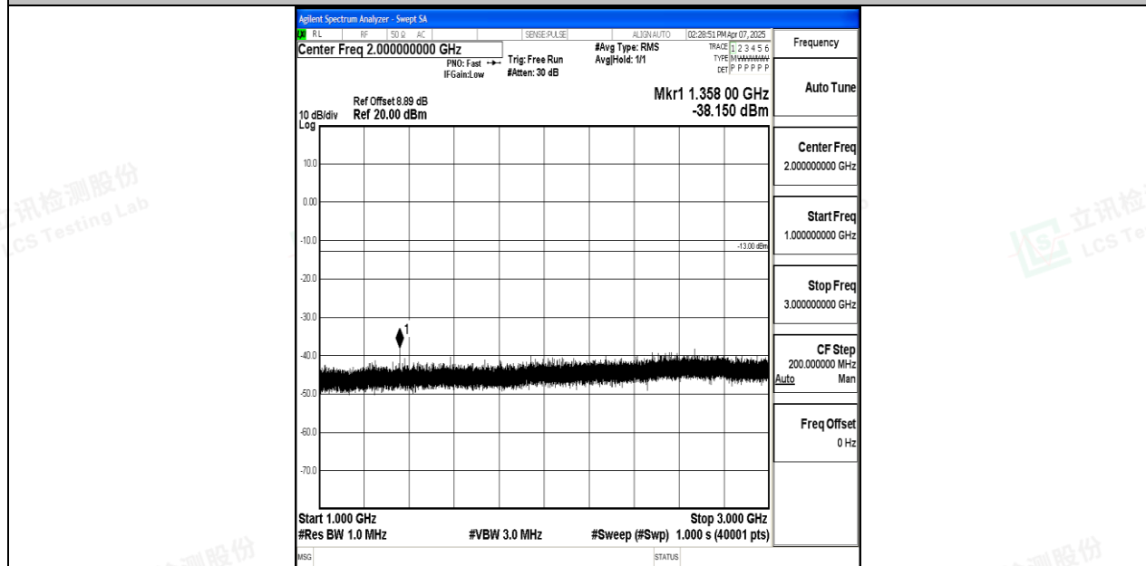
Band71_20MHz_QPSK_133372_1RB#0_1000~3000_1000~3000
