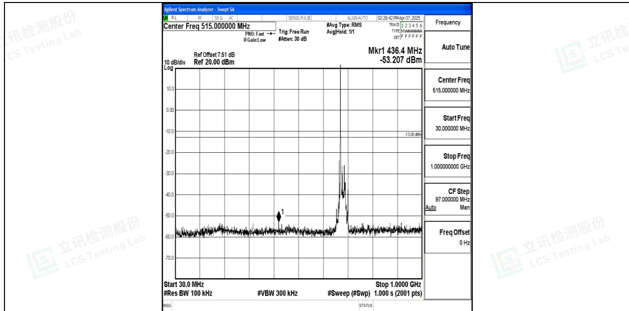
Band71_20MHz_QPSK_133372_1RB#0_30~1000_30~1000
