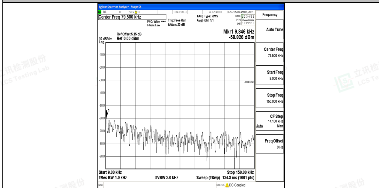
Band71_20MHz_16QAM_133322_1RB#0_0.009~0.15_0.009~0.15
