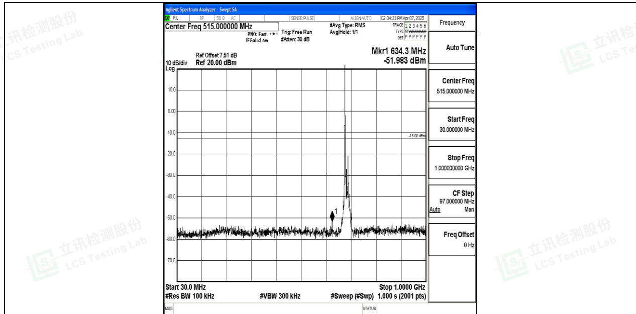
Band71_15MHz_QPSK_133397_1RB#0_30~1000_30~1000
