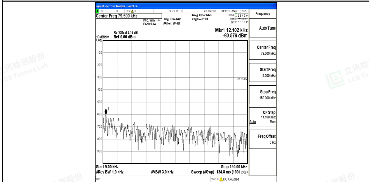
Band71_10MHz_16QAM_133422_1RB#0_0.009~0.15_0.009~0.15
