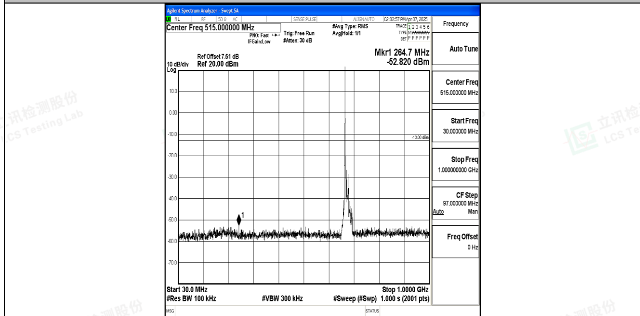
Band71_15MHz_16QAM_133297_1RB#0_30~1000_30~1000
