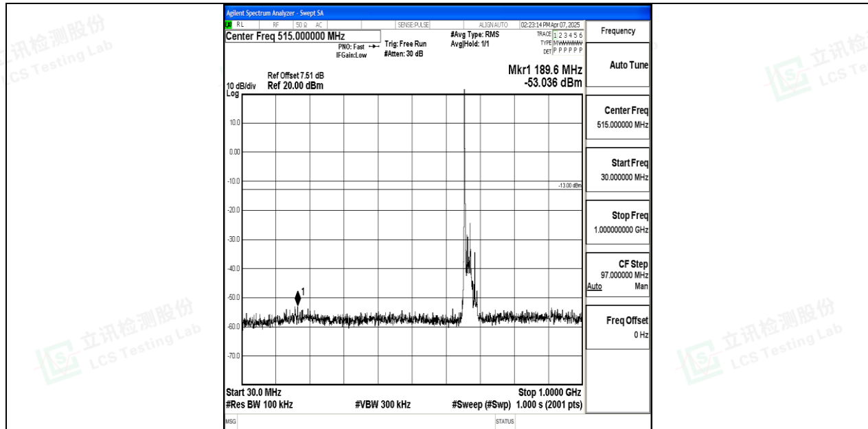
Band71_20MHz_QPSK_133222_1RB#0_30~1000_30~1000
