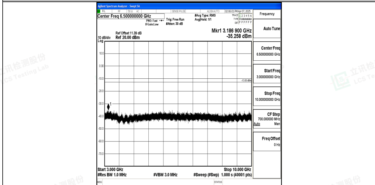
Band71_15MHz_16QAM_133397_1RB#0_3000~10000_3000~10000
