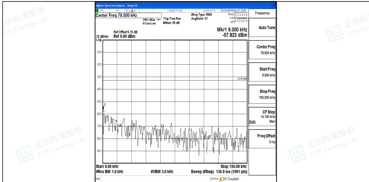
Band71_15MHz_QPSK_133397_1RB#0_0.009~0.15_0.009~0.15
