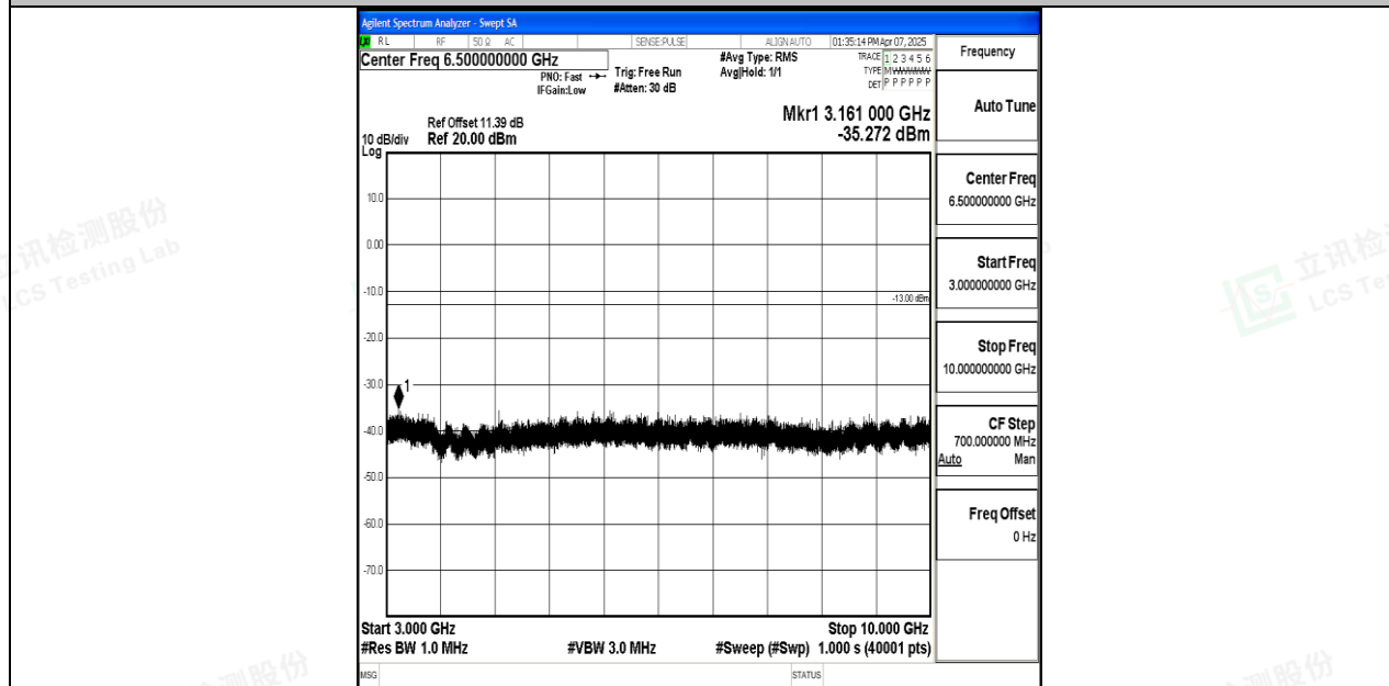
Band71_10MHz_16QAM_133172_1RB#0_3000~10000_3000~10000
