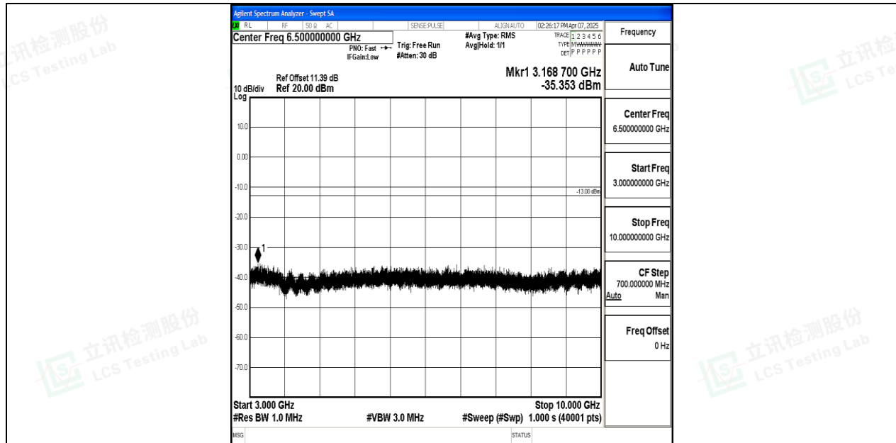
Band71_20MHz_QPSK_133322_1RB#0_3000~10000_3000~10000
