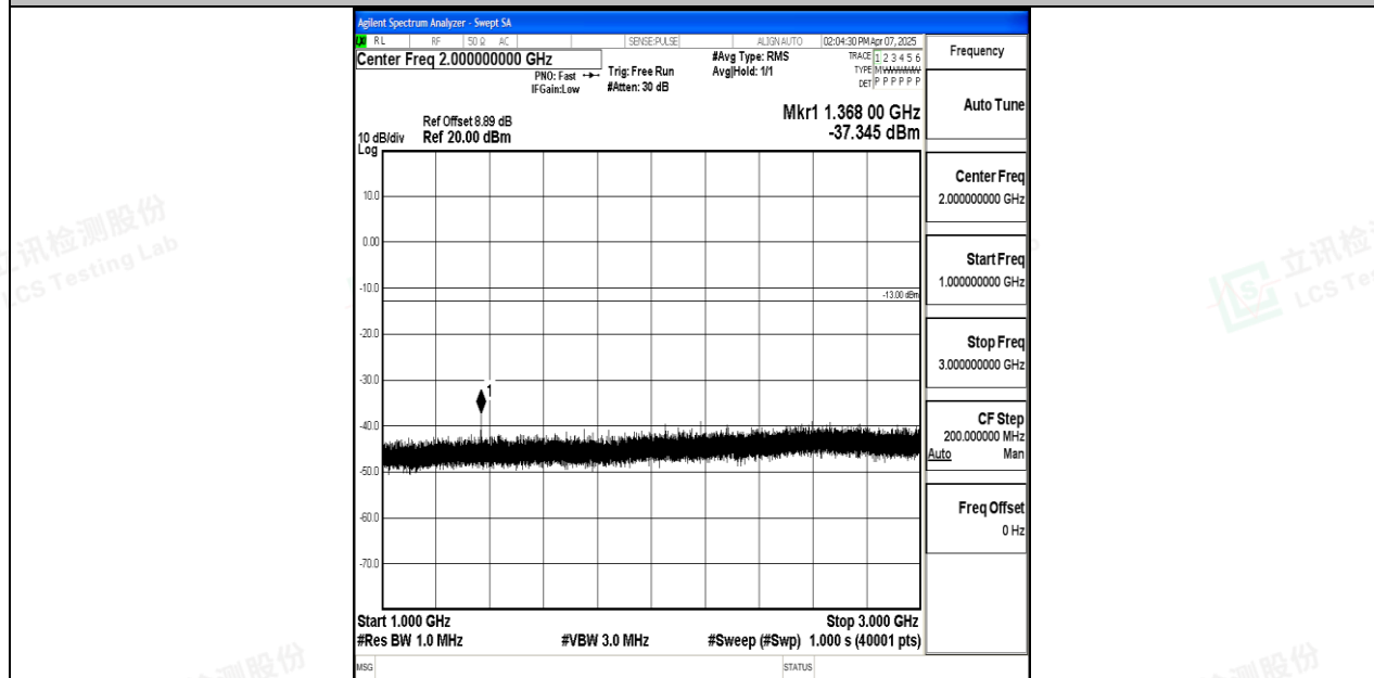
Band71_15MHz_QPSK_133397_1RB#0_1000~3000_1000~3000
