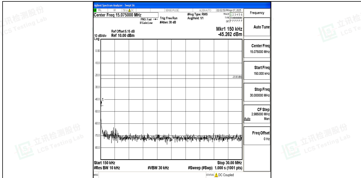
Band71_15MHz_16QAM_133297_1RB#0_0.15~30_0.15~30
