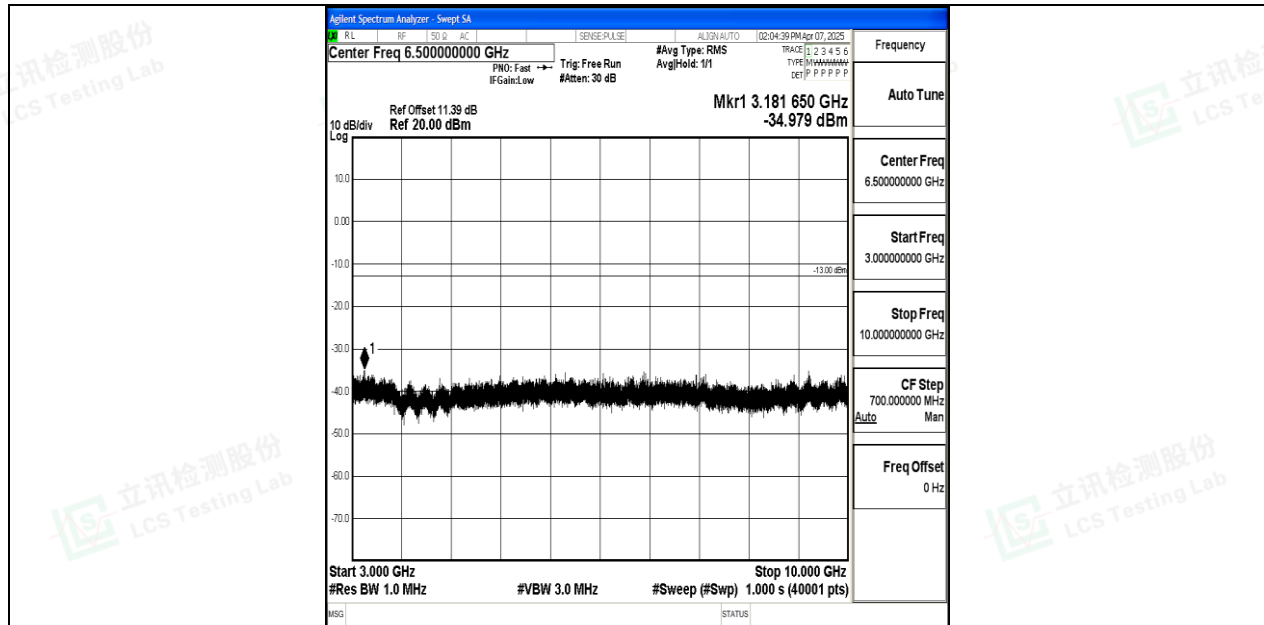
Band71_15MHz_QPSK_133397_1RB#0_3000~10000_3000~10000
