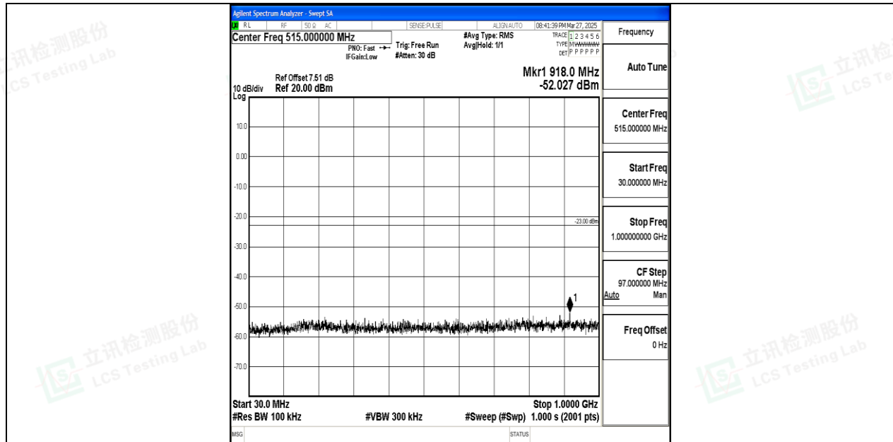
Band66_15MHz_16QAM_132322_1RB#0_30~1000_30~1000
