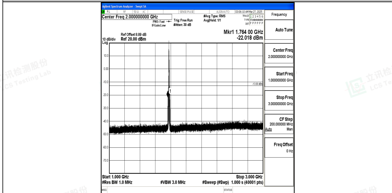
Band66_5MHz_16QAM_132647_1RB#0_1000~3000_1000~3000
