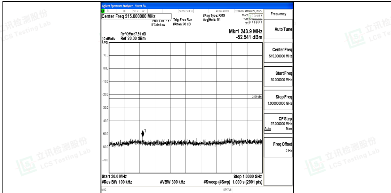
Band66_5MHz_16QAM_132647_1RB#0_30~1000_30~1000
