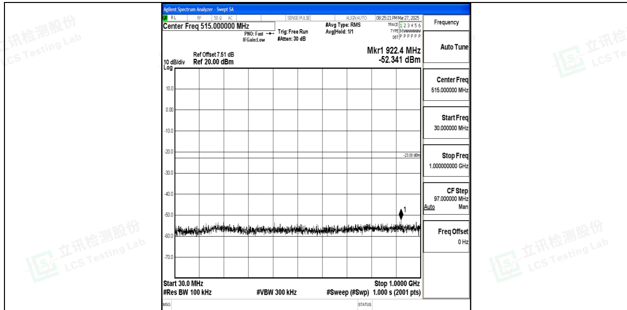
Band66_10MHz_16QAM_132622_1RB#0_30~1000_30~1000
