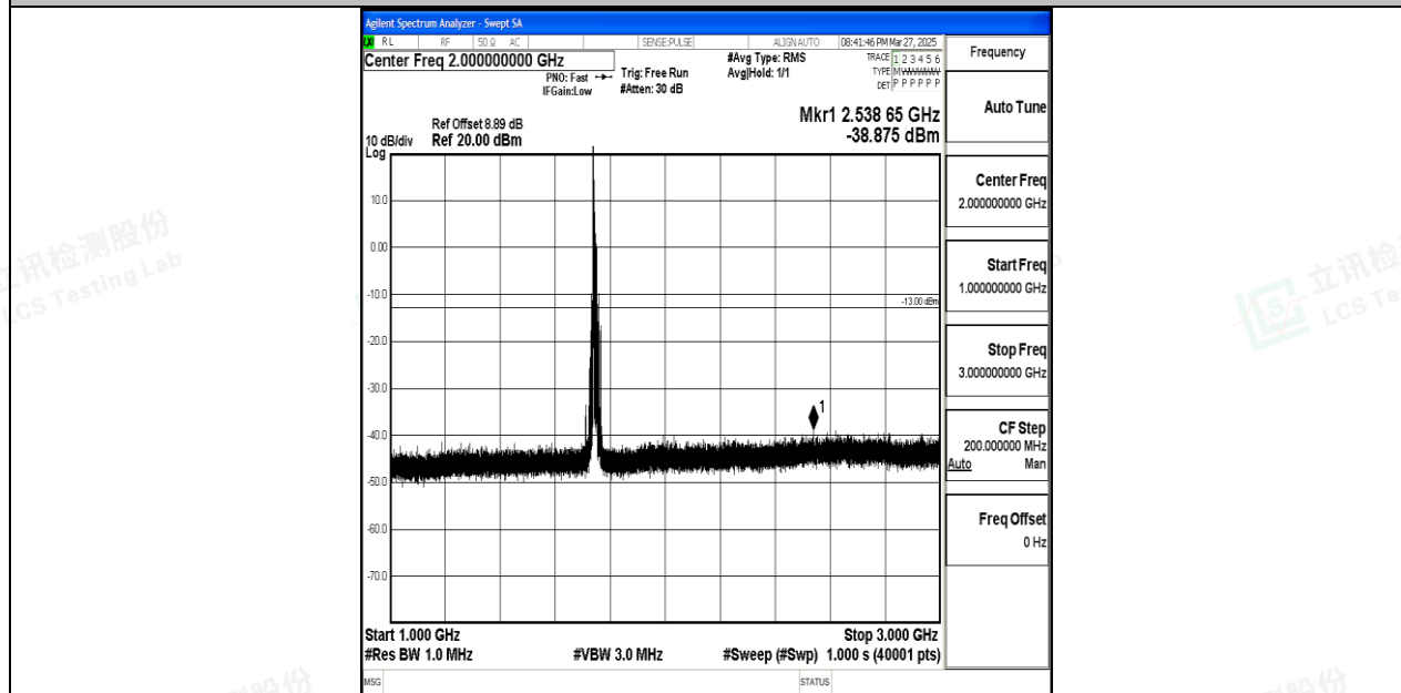
Band66_15MHz_16QAM_132322_1RB#0_1000~3000_1000~3000
