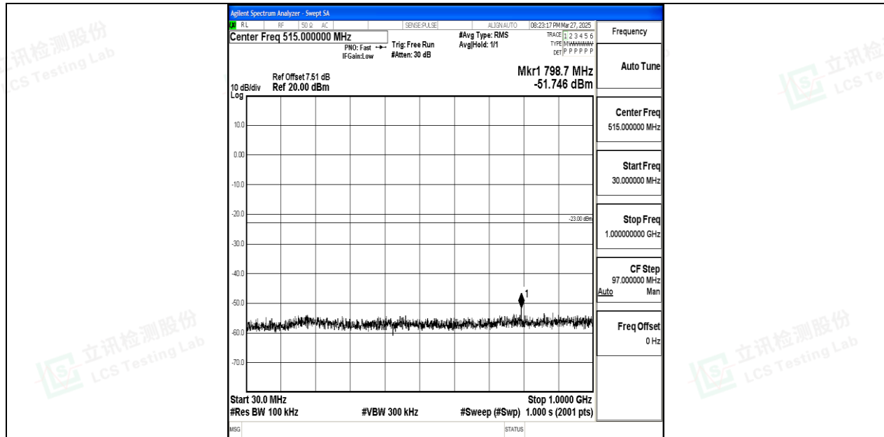
Band66_10MHz_16QAM_132022_1RB#0_30~1000_30~1000
