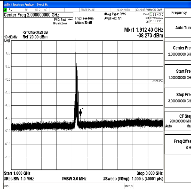
Band2_20MHz_QPSK_18700_1RB#0_1000~3000_1000~3000
