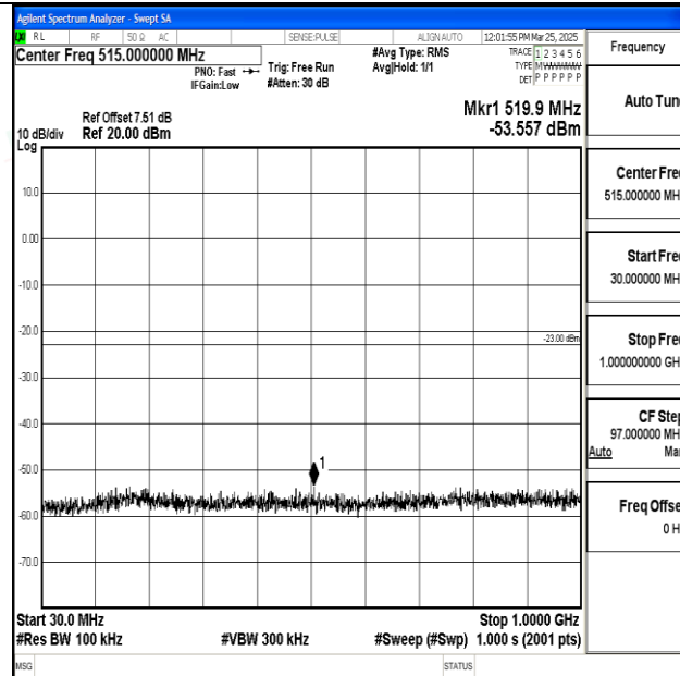
Band2_15MHz_16QAM_18900_1RB#0_30~1000_30~1000
