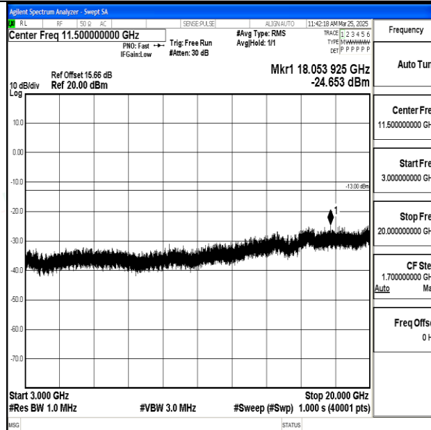
Band2_10MHz_QPSK_19150_1RB#0_3000~20000_3000~20000
