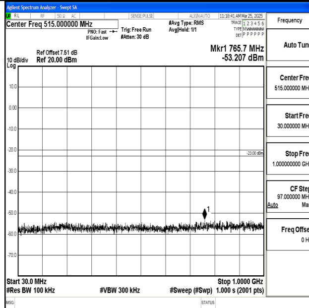
Band2_5MHz_16QAM_18900_1RB#0_30~1000_30~1000
