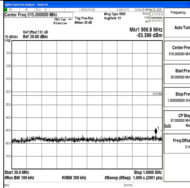
Band2_10MHz_16QAM_18900_1RB#0_30~1000_30~1000
