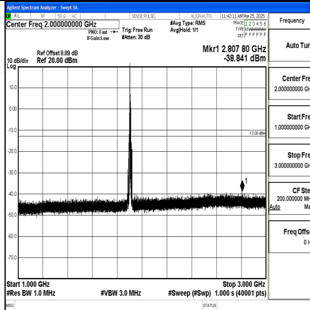
Band2_10MHz_QPSK_19150_1RB#0_1000~3000_1000~3000
