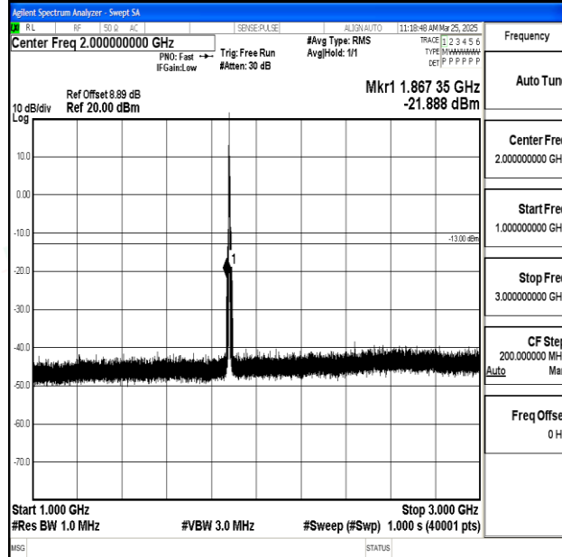
Band2_5MHz_16QAM_18900_1RB#0_1000~3000_1000~3000
