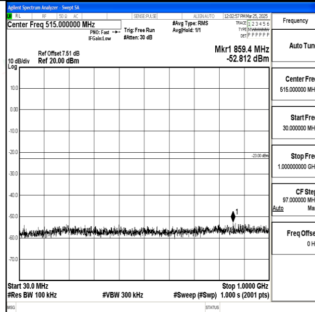
Band2_15MHz_16QAM_19125_1RB#0_30~1000_30~1000
