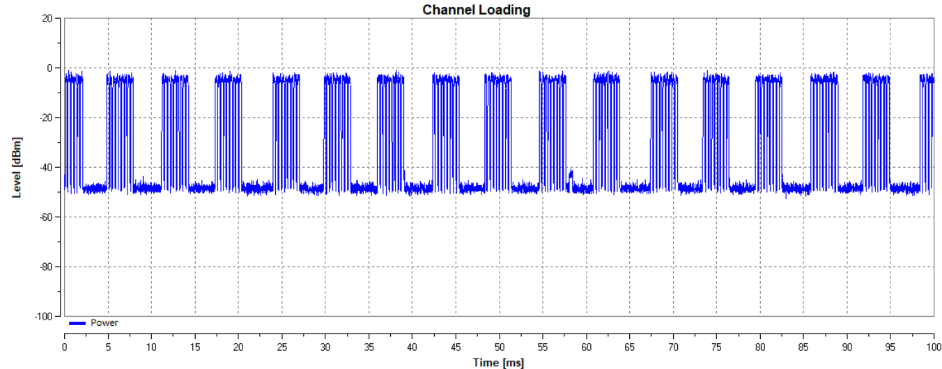
802.11n- HT40
