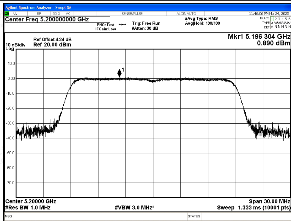
PSD NVNT n20 5200MHz Ant
