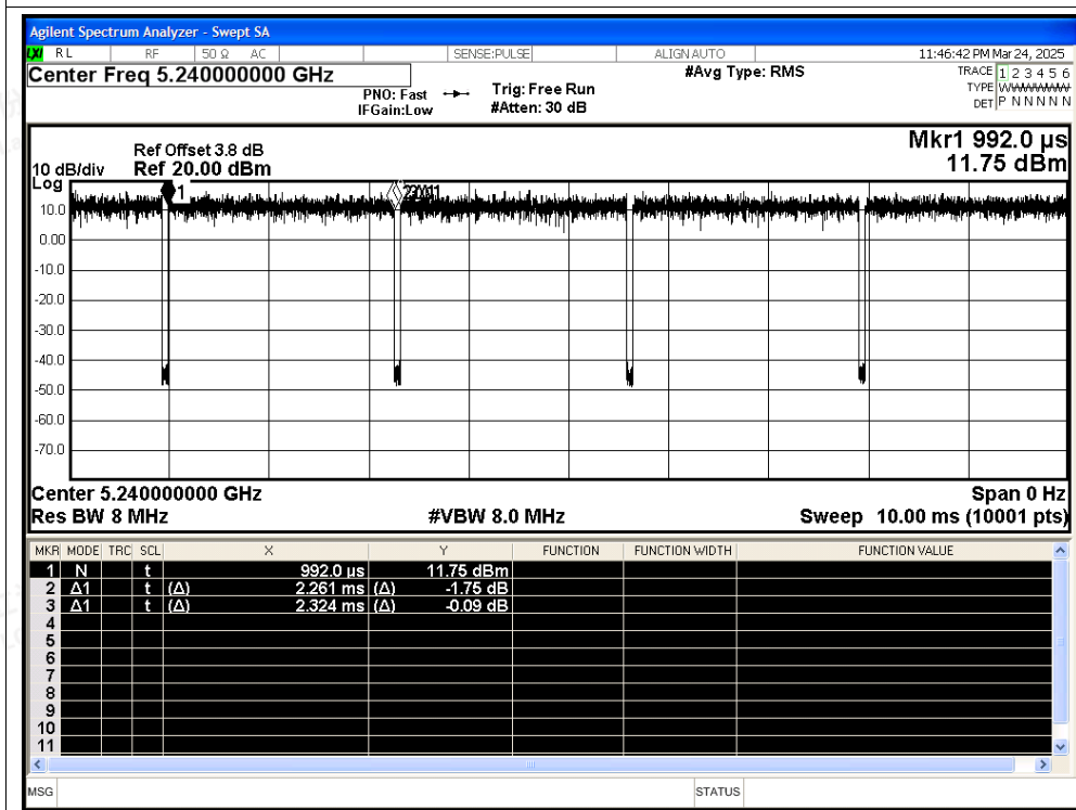
Duty Cycle NVNT n20 5240MHz Ant
