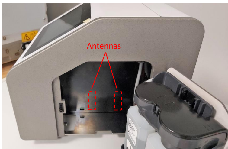
Fig. 3 - opened fluid/liquid bottles compartment (PE RFID antennas behind black plastic cover)
