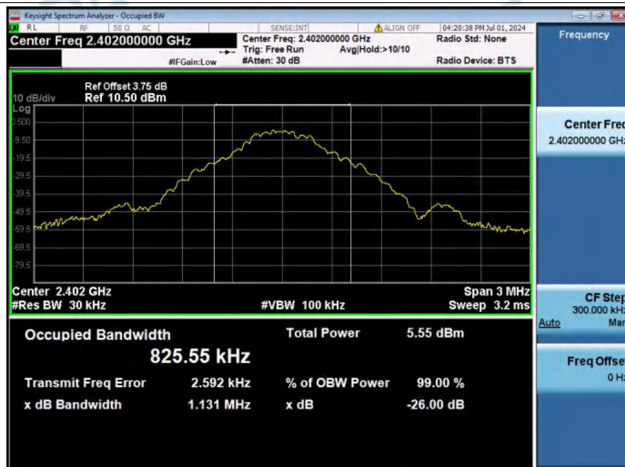
99%_Occupied_Bandwidth_NVNT_ANT1_1-DH5_2402_00
