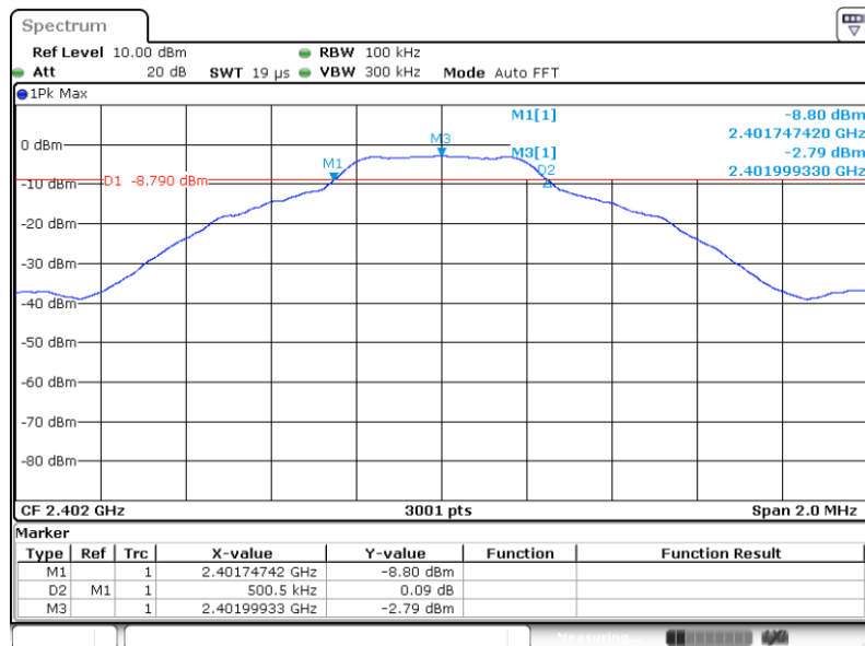
1M_LCH_2402MHz_Ant1_NTNV
