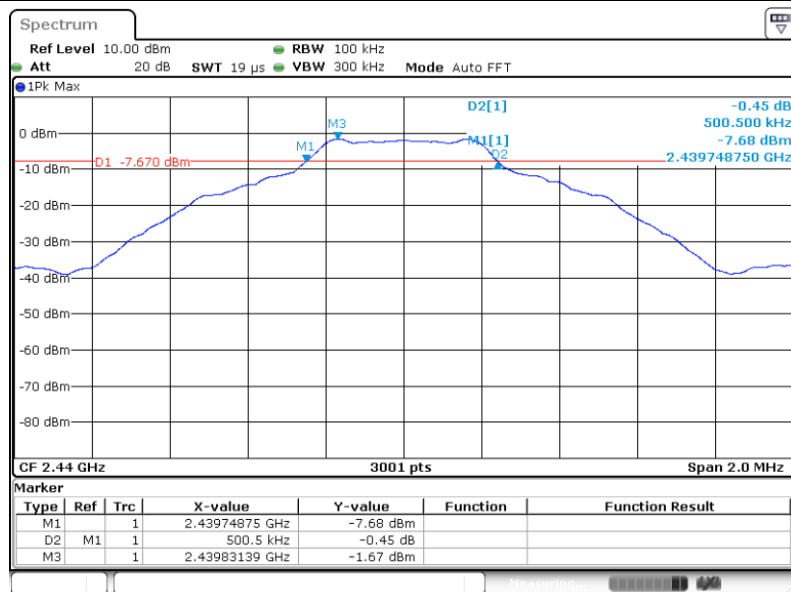
1M_MCH_2440MHz_Ant1_NTNV
