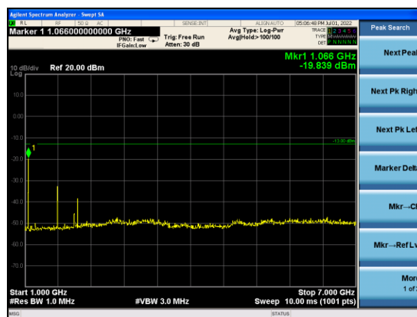
TX CH16(1GHz-7GHz)
