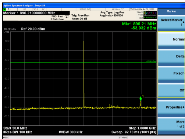
TX CH08(30MHz-1GHz)
