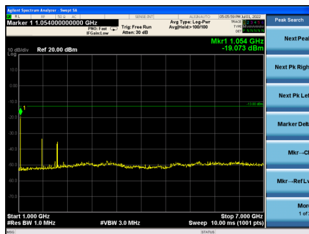
TX CH16(1GHz-7GHz)
