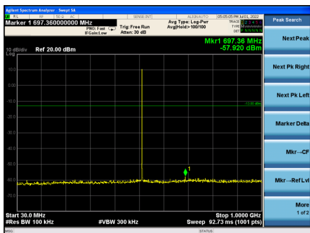
TX CH16(30MHz-1GHz)
