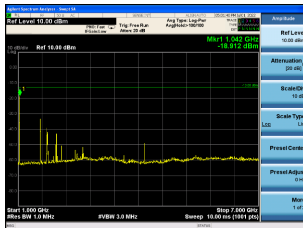
TX CH08(1GHz-7GHz)
