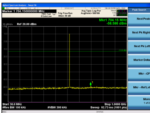
TX CH16(30MHz-1GHz)
