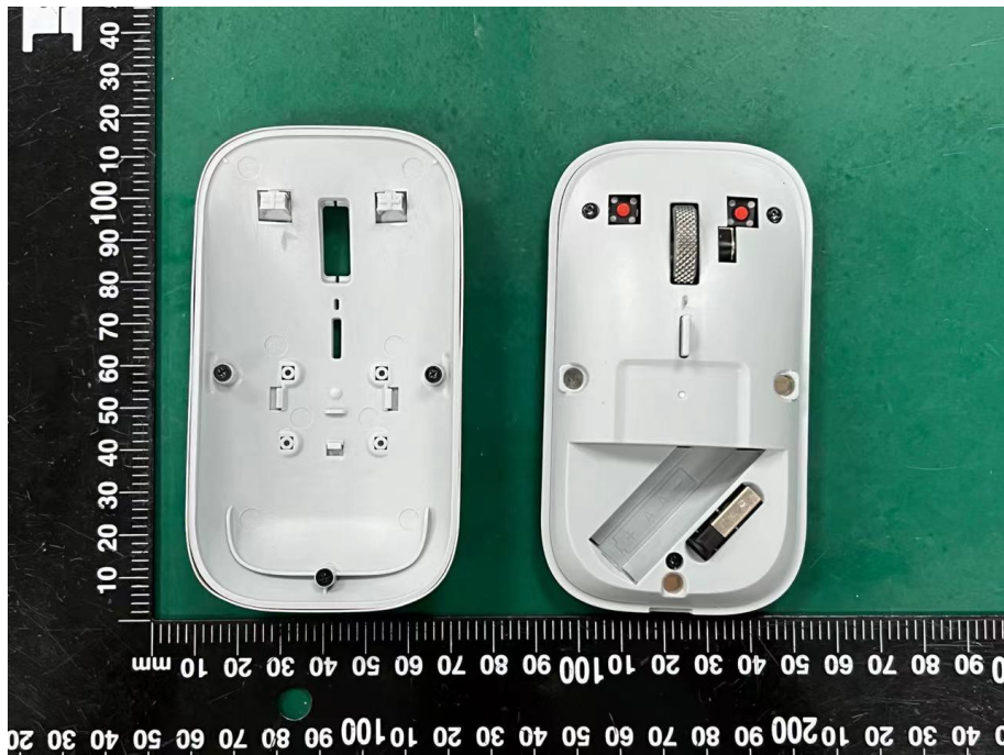
Internal Photo FCC ID: 2A692-M202
