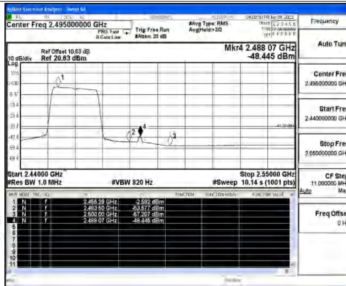
11N20ISO_Ant1_High_2462_Peak
