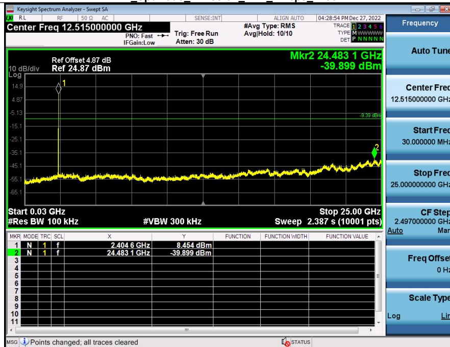
2 Spurious_Emission_BLE_1Mbps_2405
