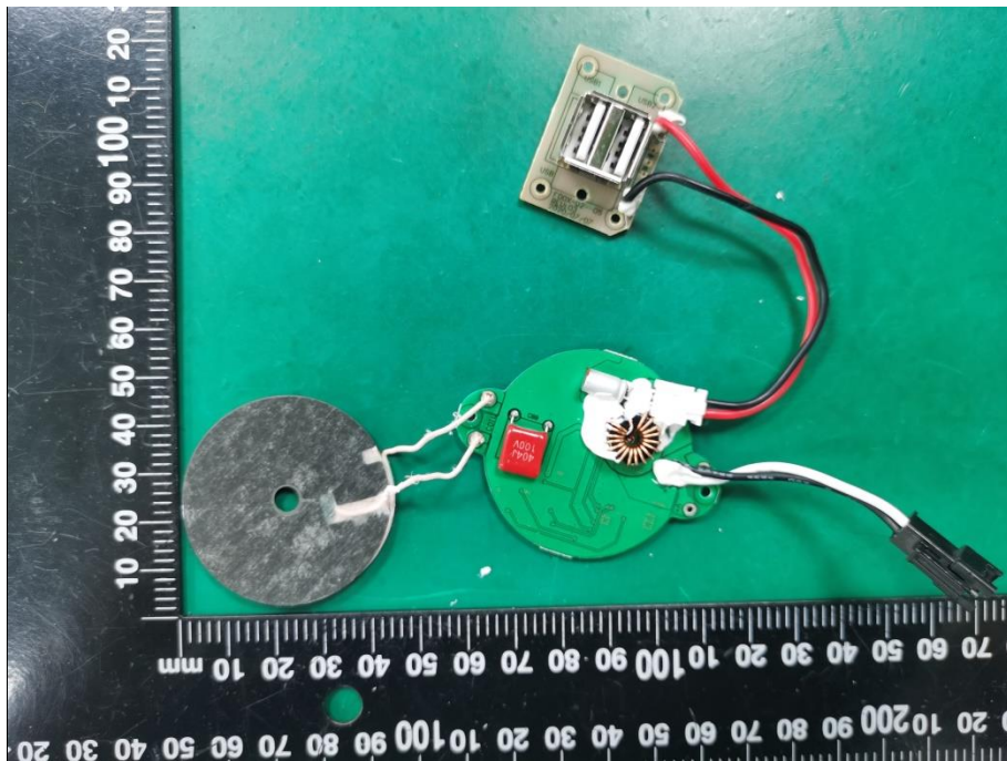
Internal Photo FCC ID: 2A68H-YY134
