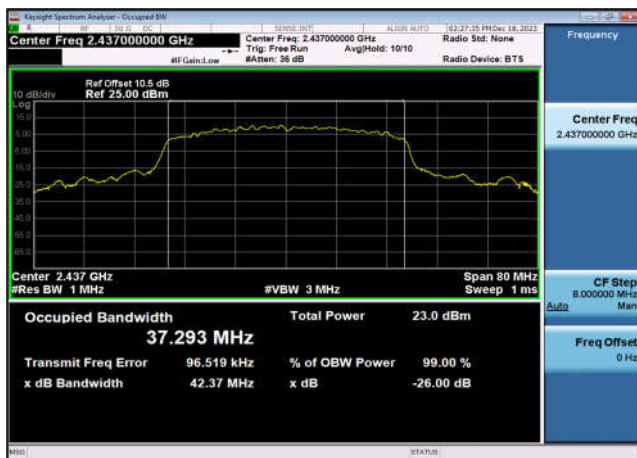
99% Bandwidth-802.11ax(HE40),2437MHz ,Ant0
