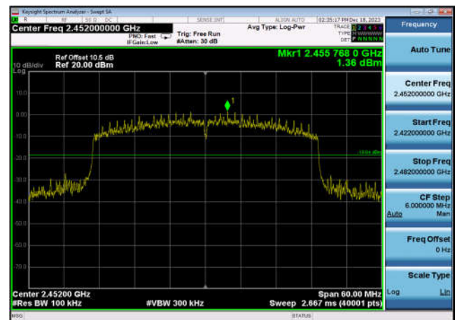
,Plot 1,Reference Level-802.11ax(HE40 ) ,2452MHz,Ant0
