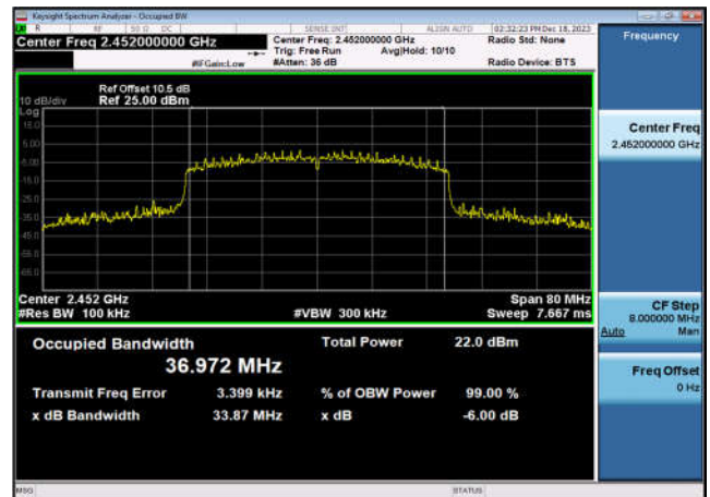
6dB Bandwidth-802.11ax(HE40),2452MHz ,Ant0
