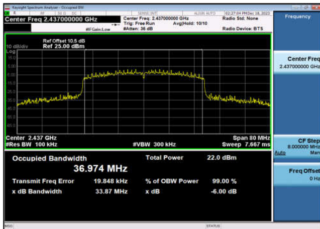
6dB Bandwidth-802.11ax(HE40),2437MHz ,Ant0
