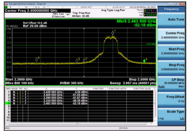
,Plot 2,Band Edge-802.11ax(HE40) ,2422MHz,Ant0
