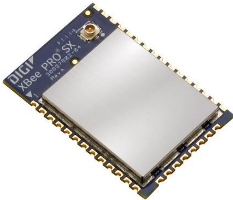
Figure 1 - Radio Module - External - Top, Angled View
