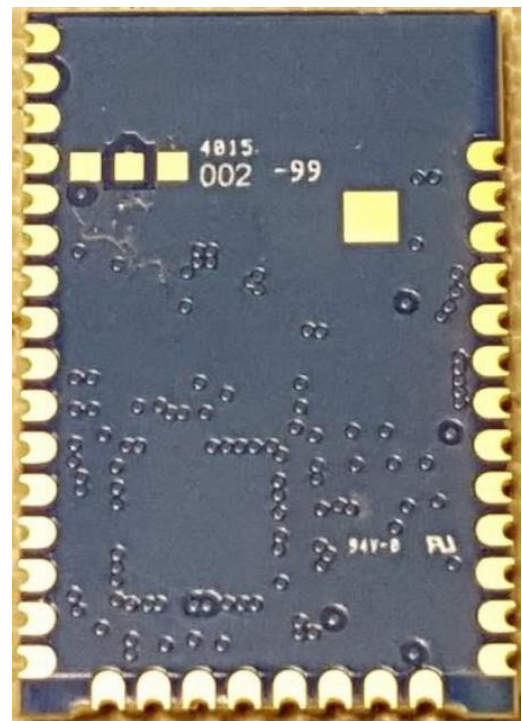
Figure 3 - Radio Module - External - Bottom View
