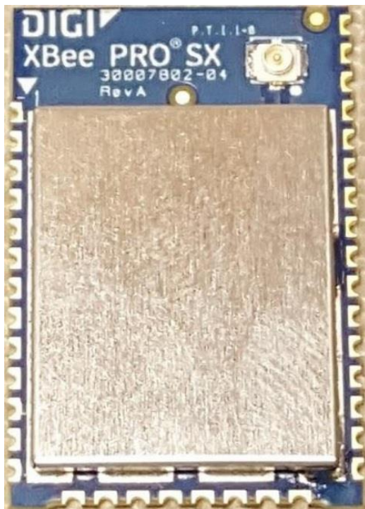
Figure 2 - Radio Module - External - Top View
