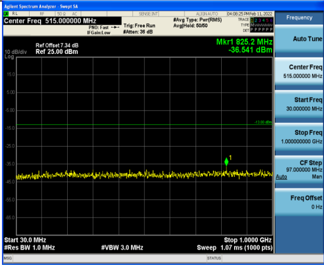
Band4-15MHz-16QAM-20325-1RB#0-Range3:30~1000MHz
