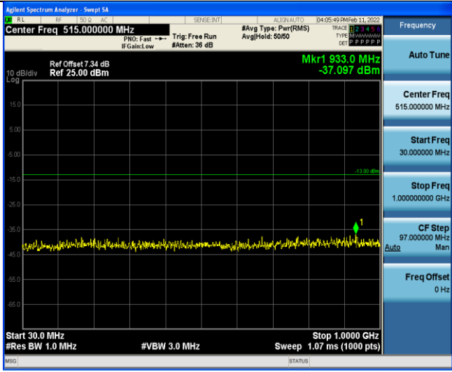
Band4-15MHz-16QAM-20025-1RB#0-Range3:30~1000MHz
