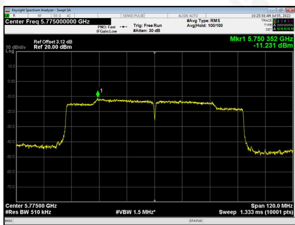
ANT2 (802.11ac80) PSD plot on channel 155
