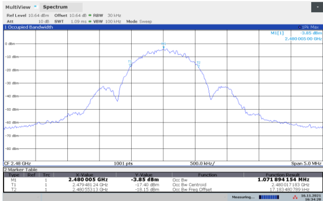
99% Occupied BW, GFSK,ch2480MHz
