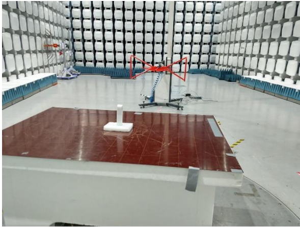
Radiated Emissions < 1GHz
