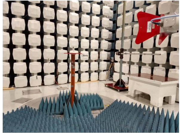
Radiated Emissions > 1GHz
