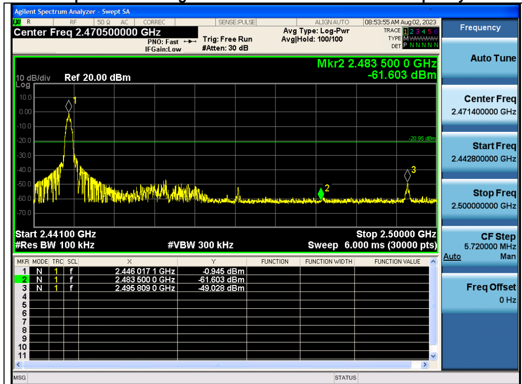
Test_Graph_ANT1_2446Mbps_Higher Band Edge Emissions
