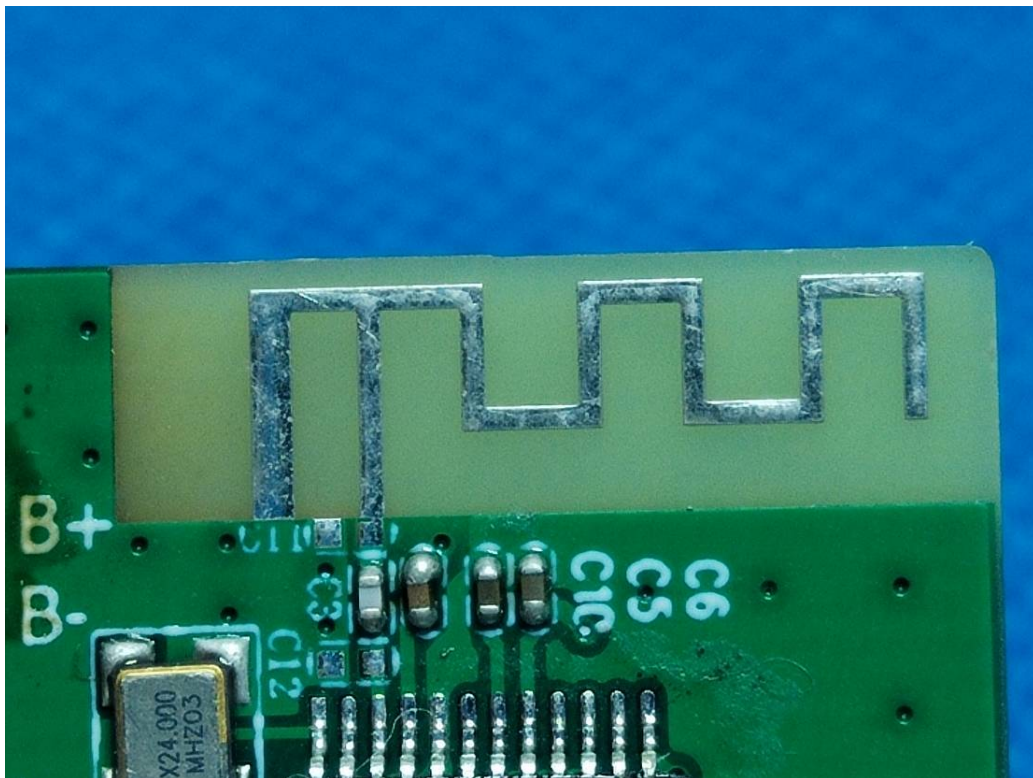
BT Antenna
