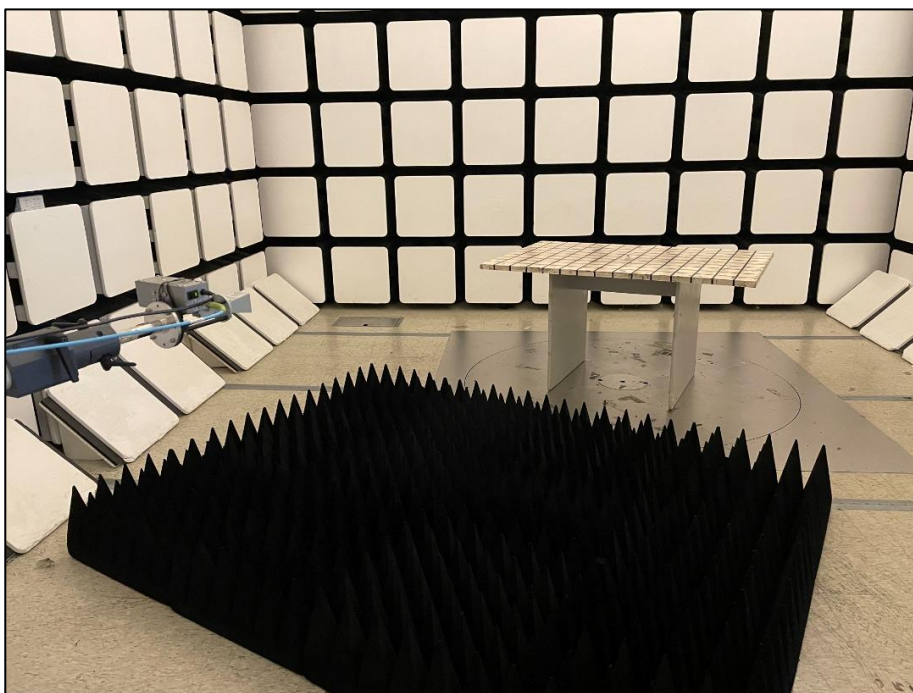
Photo 3: Measurement for 18 GHz to 40 GHz
