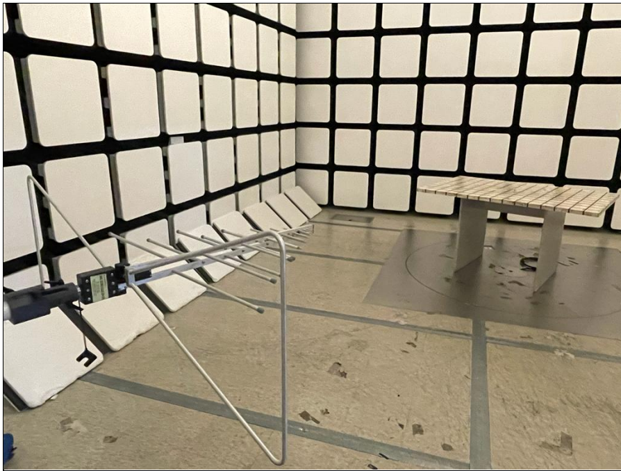
Photo 1: Measurement for 30 MHz to 1 GHz
