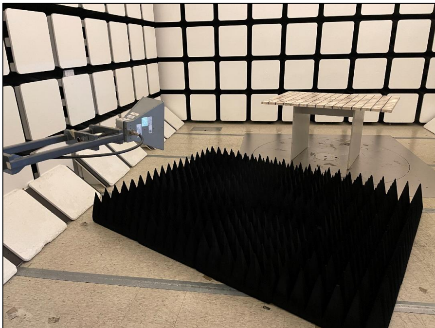
Photo 2: Measurement for 1 GHz to 18 GHz
