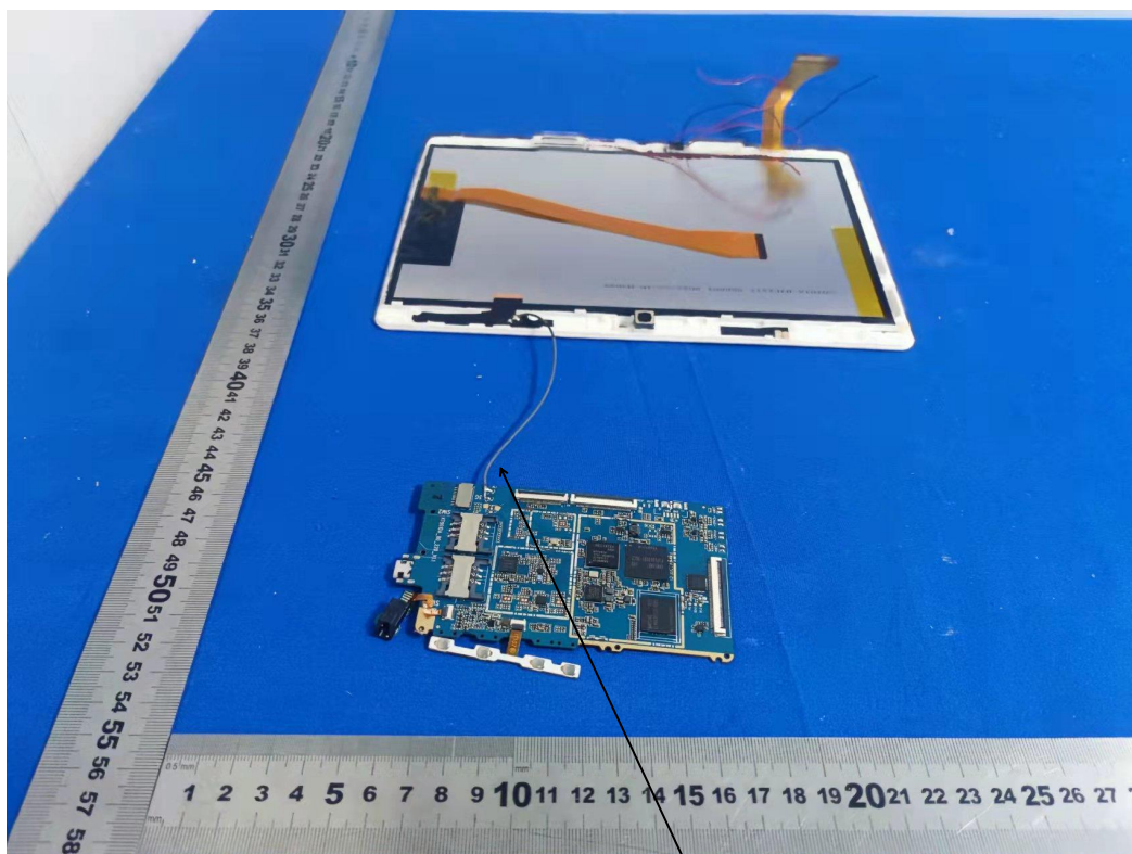
Integral Antenna
