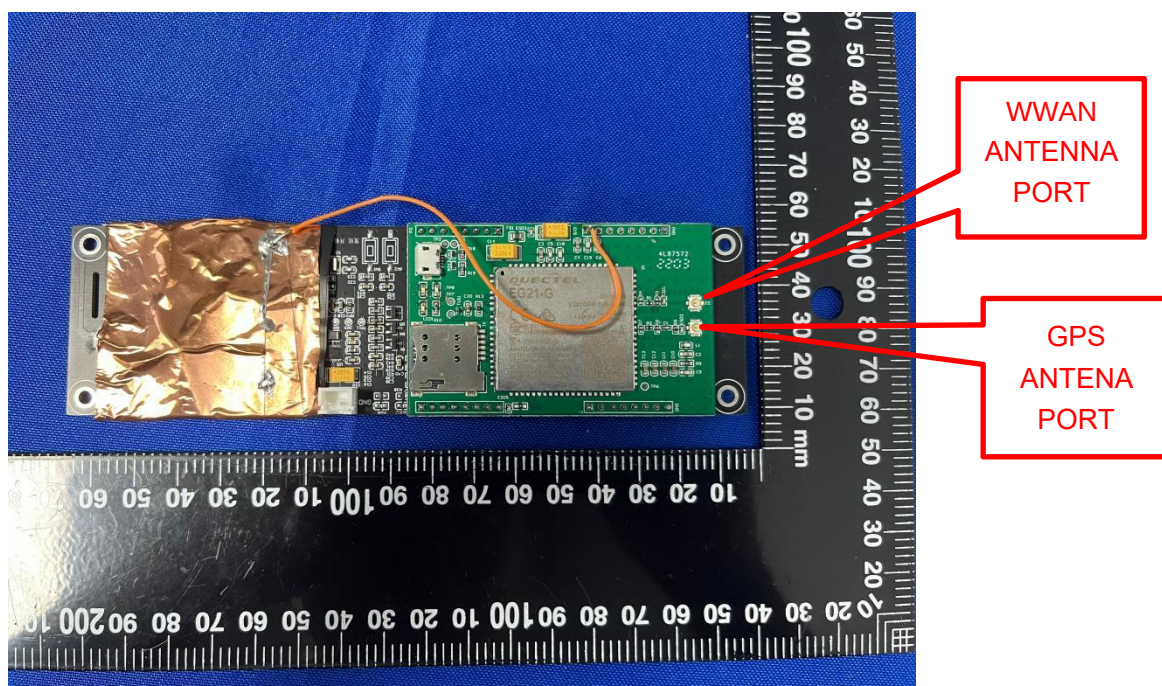
MAIN BOARD TOP VIEW (WITH SHIELDING)
