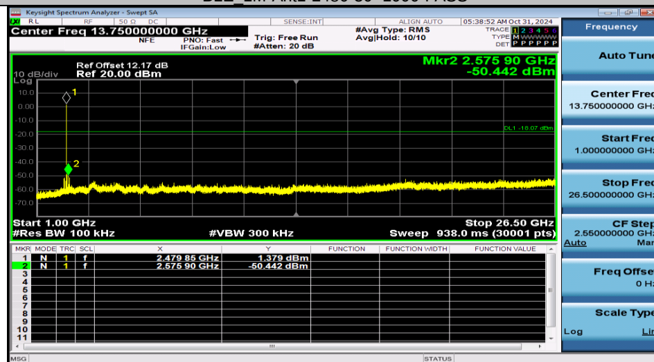
BLE_1M-Ant1-2480-1000-26500-PASS
