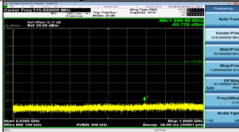
BLE_1M-Ant1-2480-30-1000-PASS
