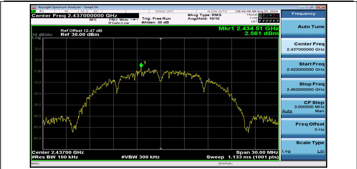
11B-Ant1-2437-0~Reference-PASS
