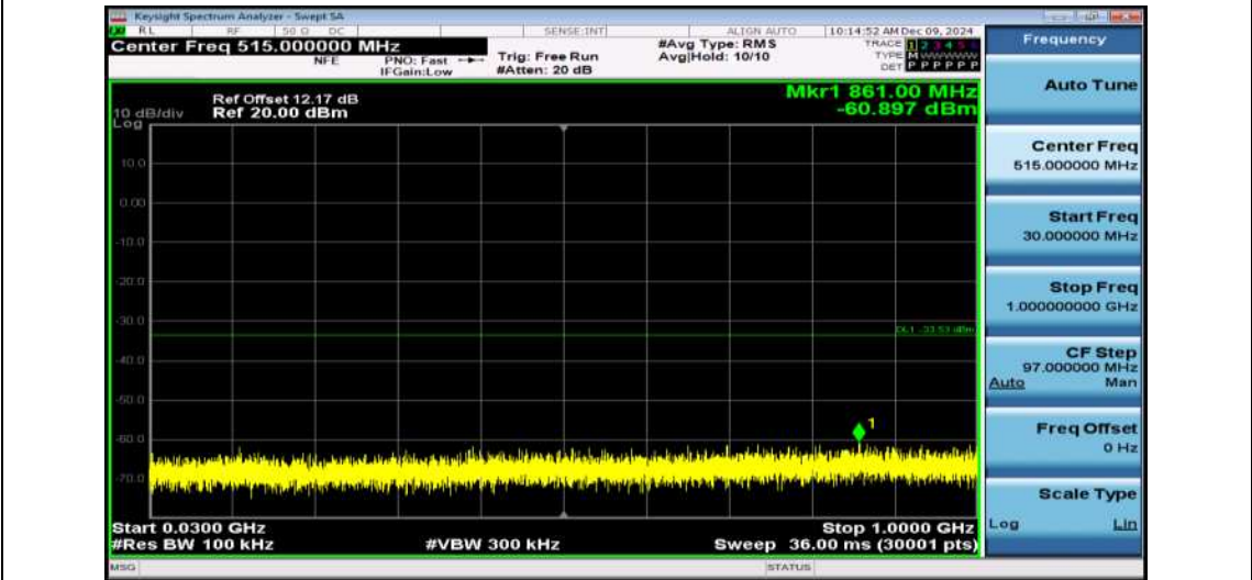
11N40SISO-Ant1-2422-30~1000-PASS
