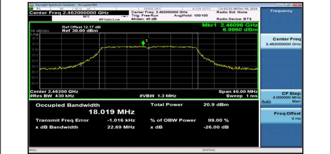
11N20SISO-Ant1-2462
