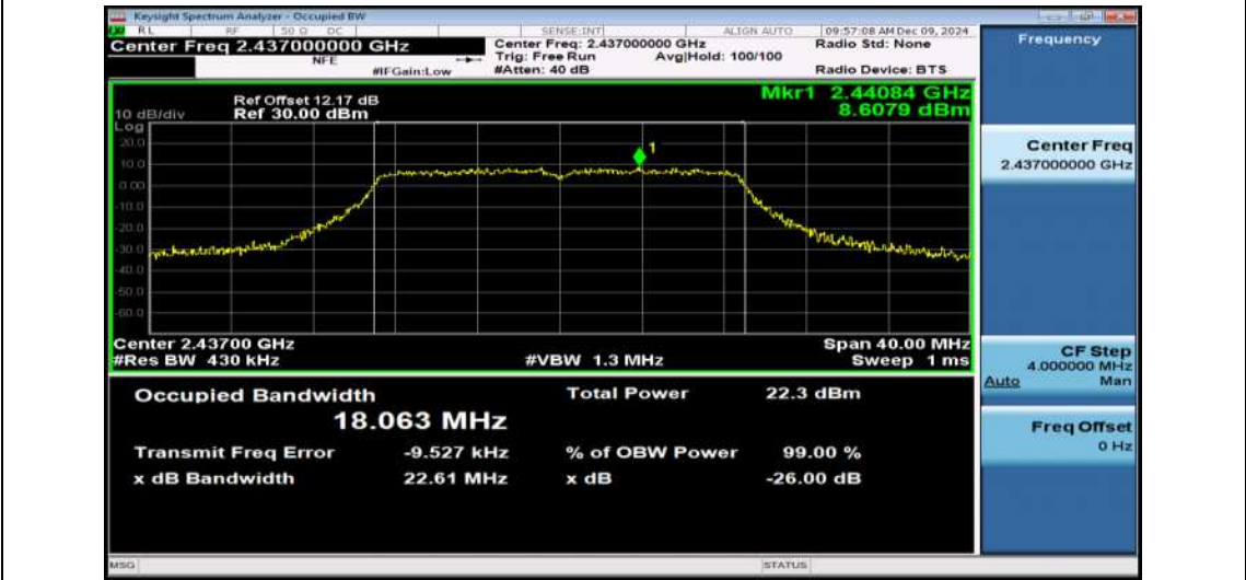
11N20SISO-Ant1-2437
