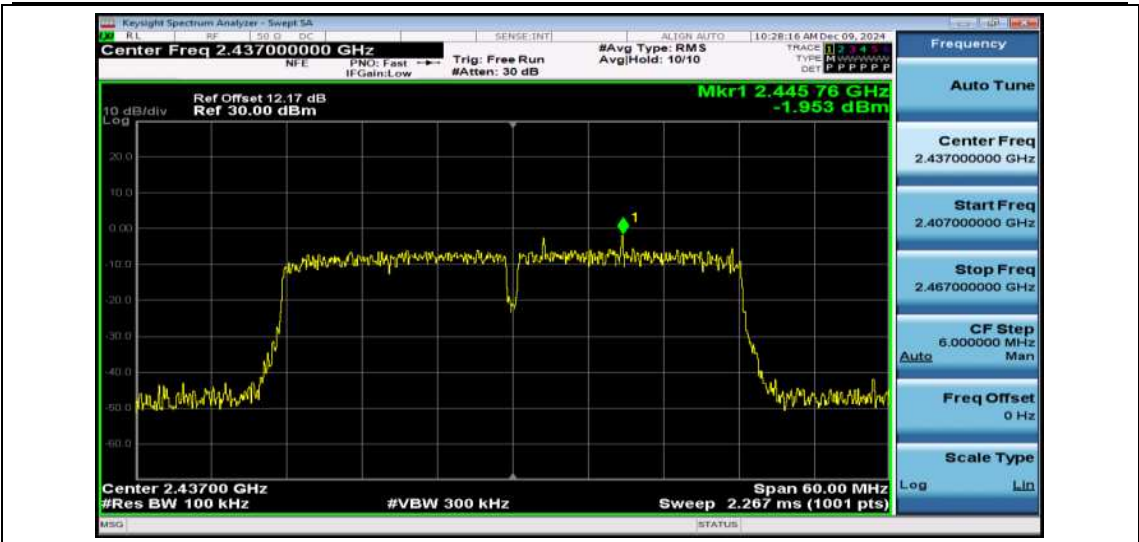
11N40SISO-Ant1-2437-0~Reference-PASS
