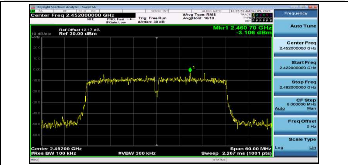
11N40SISO-Ant1-2452-0~Reference-PASS
