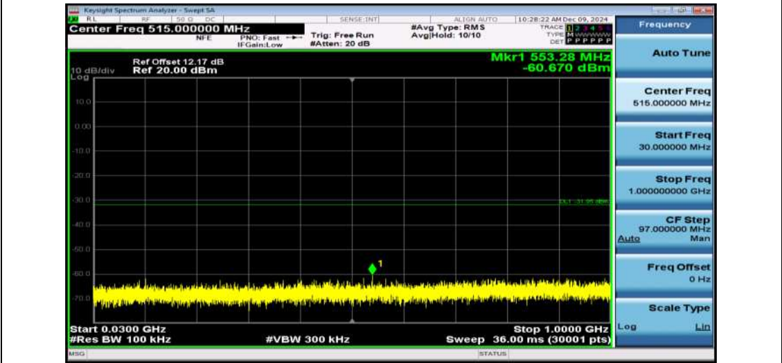
11N40SISO-Ant1-2437-30~1000-PASS
