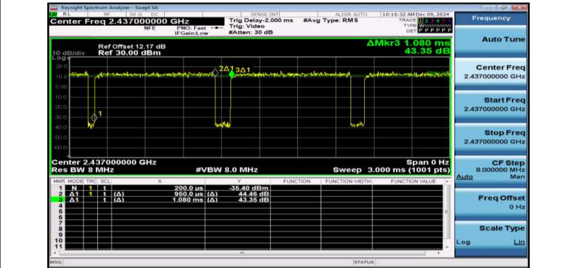
NTNV-11N40SISO-Ant1-2437
