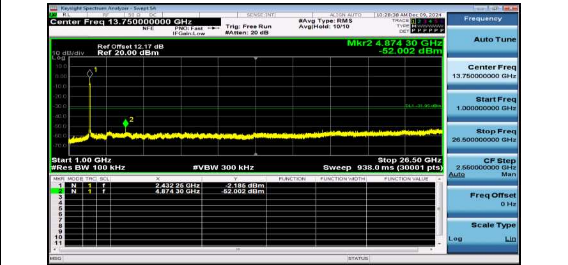
11N40SISO-Ant1-2437-1000~26500-PASS
