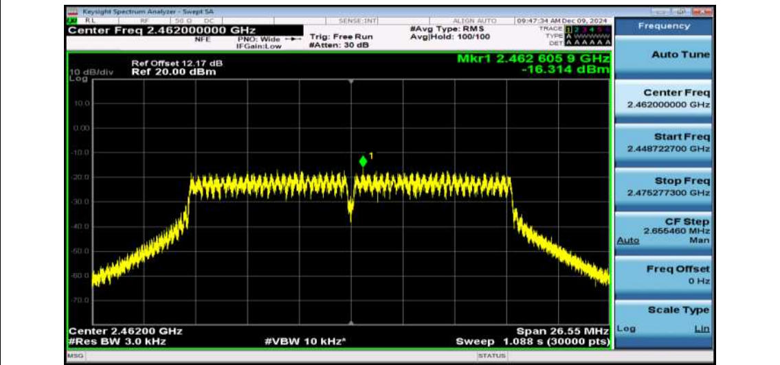
11G-Ant1-2462-PASS
