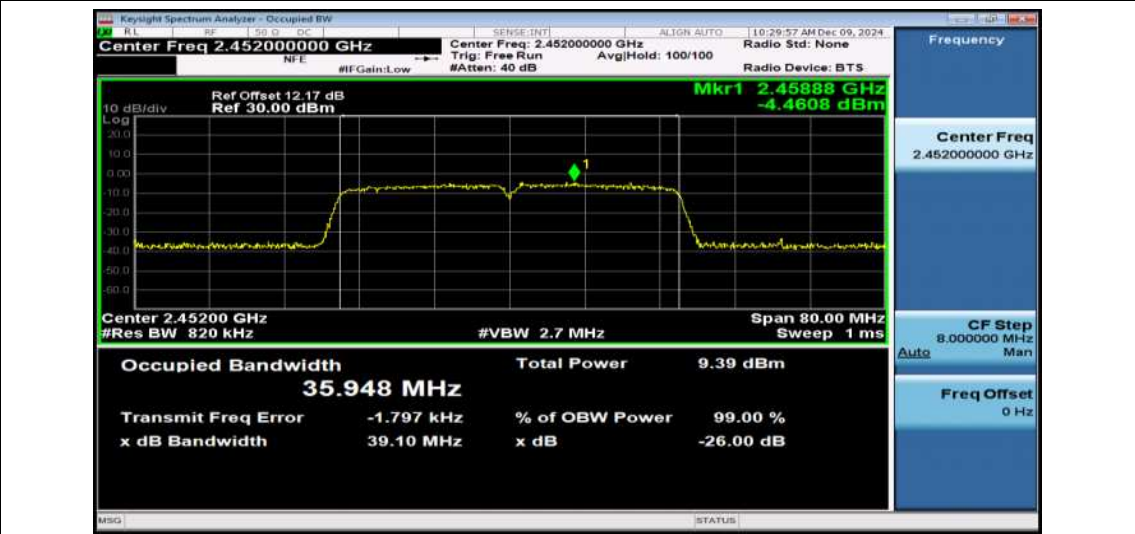
11N40SISO-Ant1-2452
