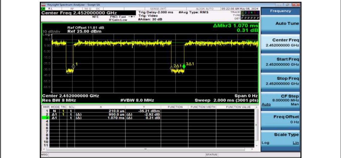
NTNV-11N40SISO-Ant1-2452
