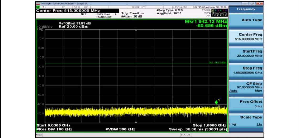
11B-Ant1-2462-30~1000-PASS
