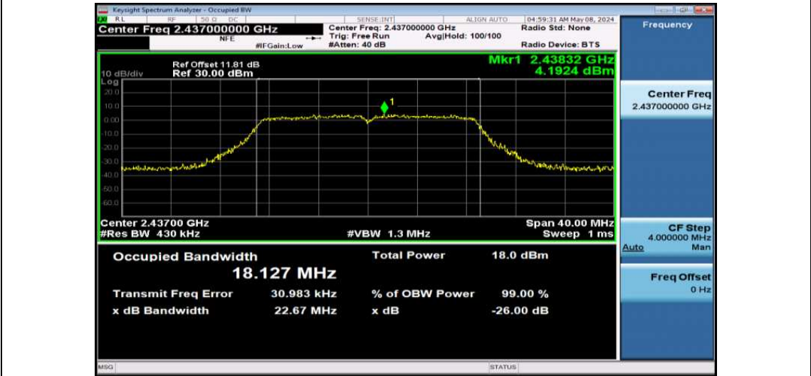
11N20SISO-Ant1-2437
