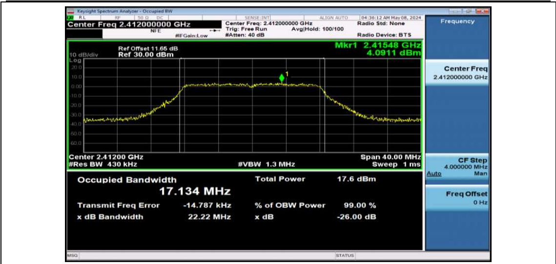
11G-Ant1-2412
