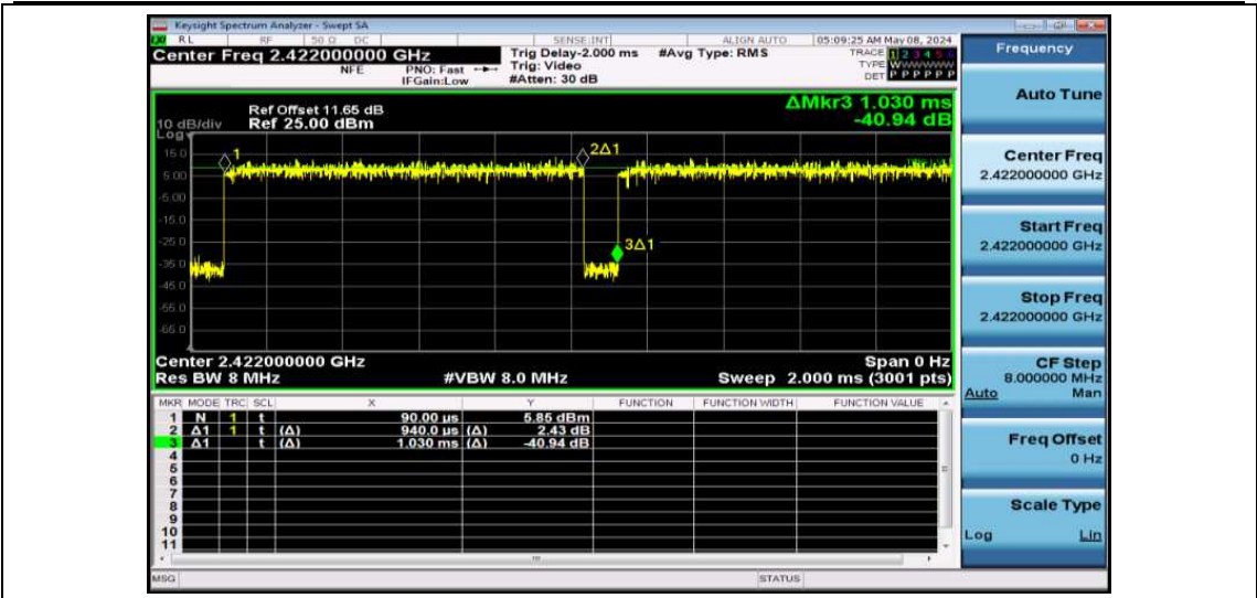
NTNV-11N40SISO-Ant1-2422
