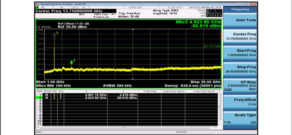
11B-Ant1-2462-1000~26500-PASS
