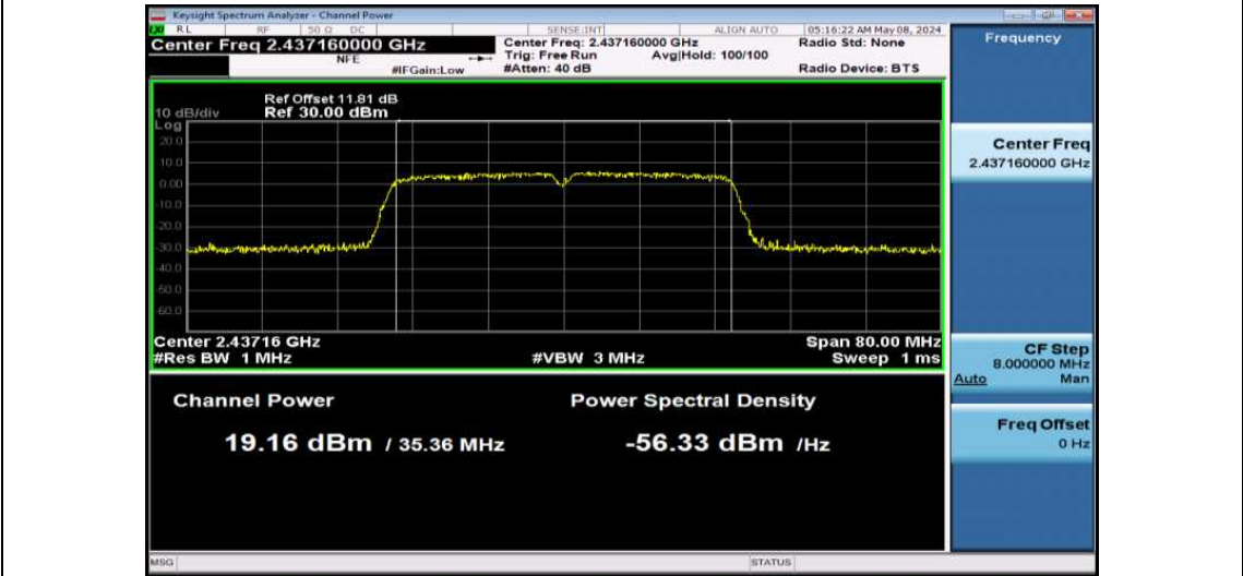
11N40SISO-Ant1-2437-PASS
