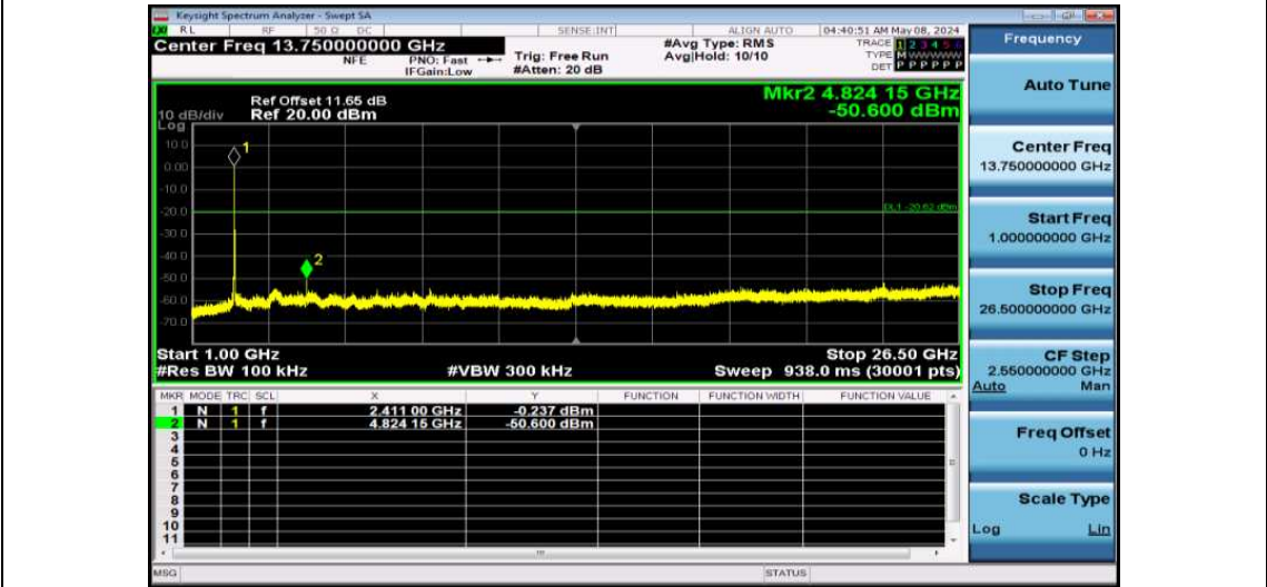
11G-Ant1-2412-1000~26500-PASS
