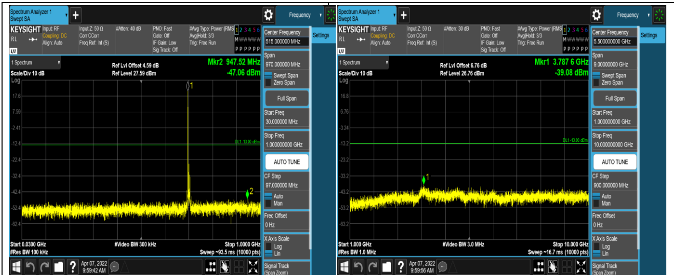
Band17-10MHz-QPSK-23790-1RB#0-Range1:30~1000
