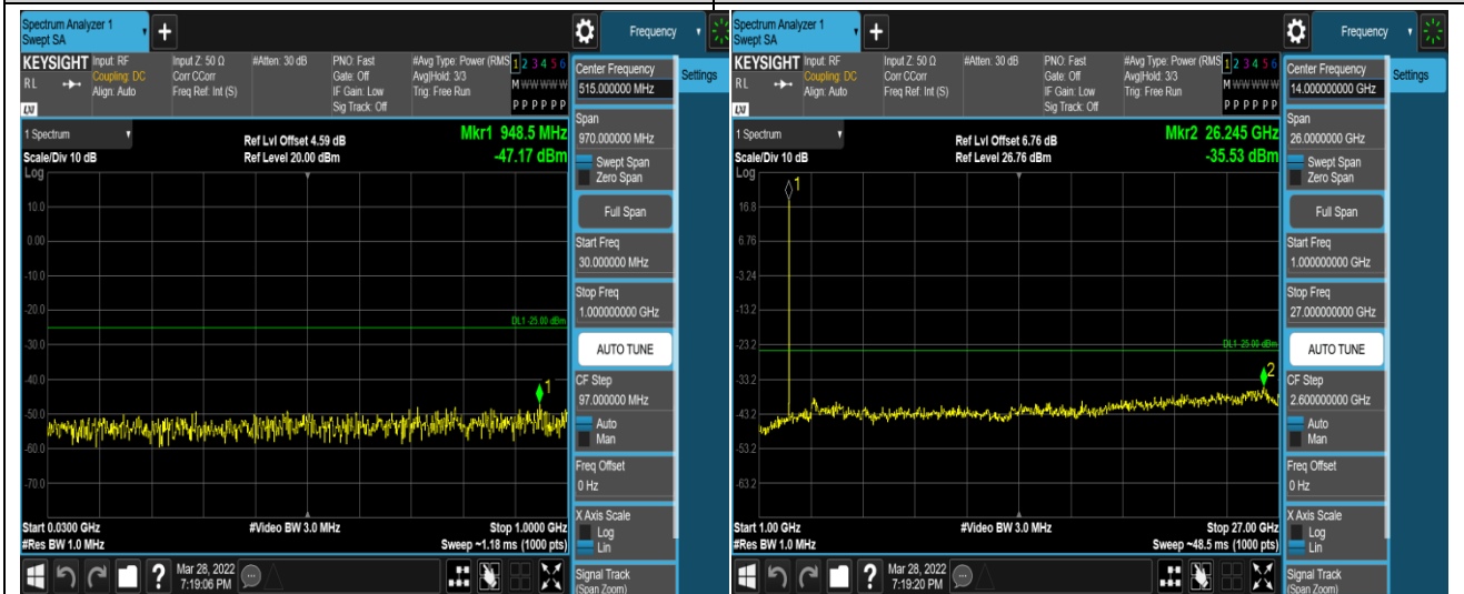
Band7-20MHz-16QAM-21100-1RB#0-Range1:30~1000
