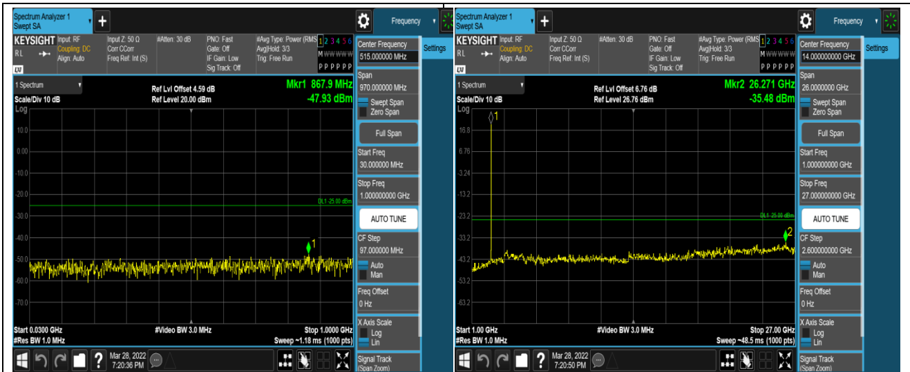
Band7-20MHz-16QAM-20850-1RB#0-Range1:30~1000
