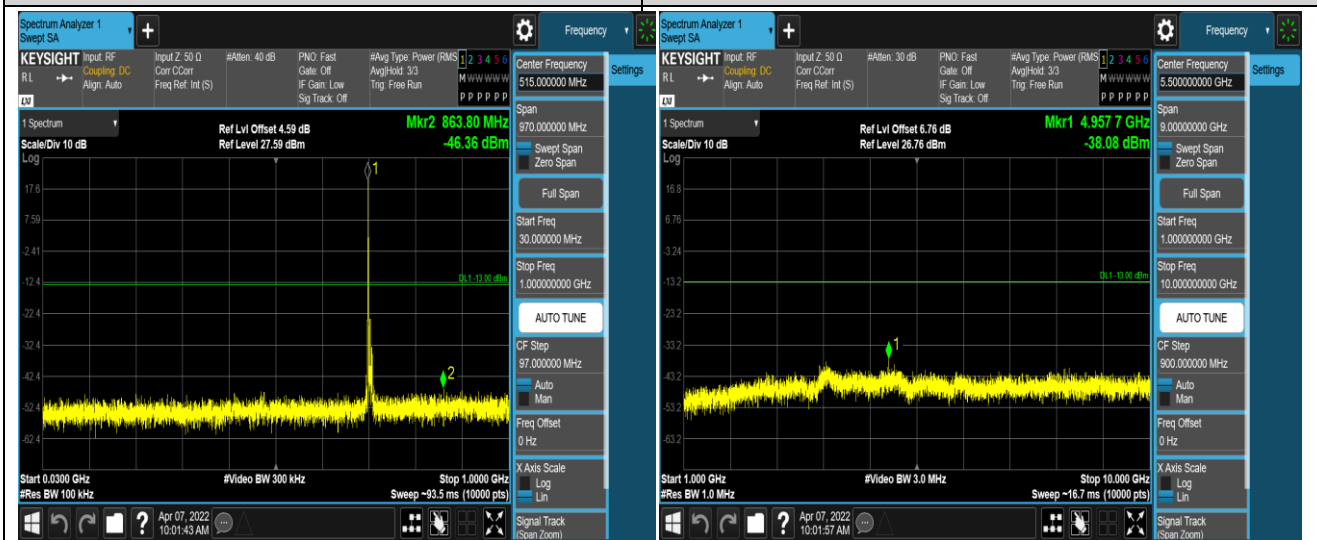
Band17-10MHz-QPSK-23800-1RB#0-Range1:30~1000
