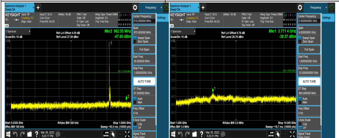
Band5-10MHz-QPSK-20525-1RB#0-Range1:30~1000M
