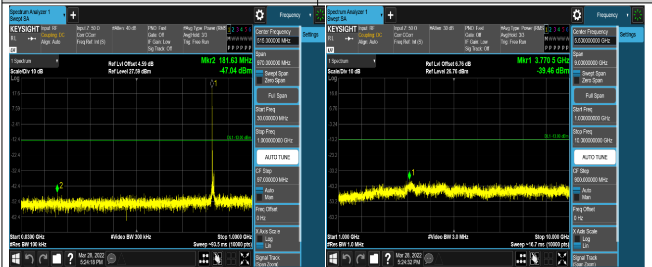
Band5-10MHz-QPSK-20525-1RB#0-Range1:30~1000M
