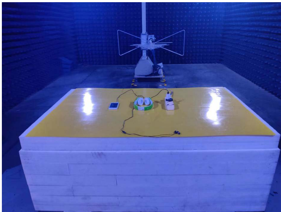
Photo of Radiated Emission Measurement Below 1GHz Model: bs690
