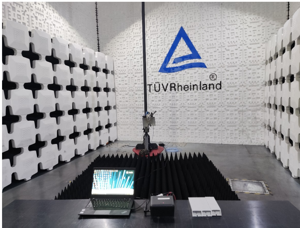
Photograph 5: Set-up photo for Radiated Emission, Above 1GHz
