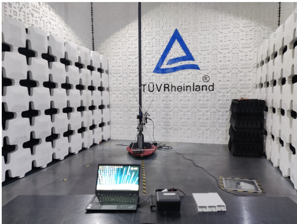
Photograph 4: Set-up photo for Radiated Emission, Below 1GHz
