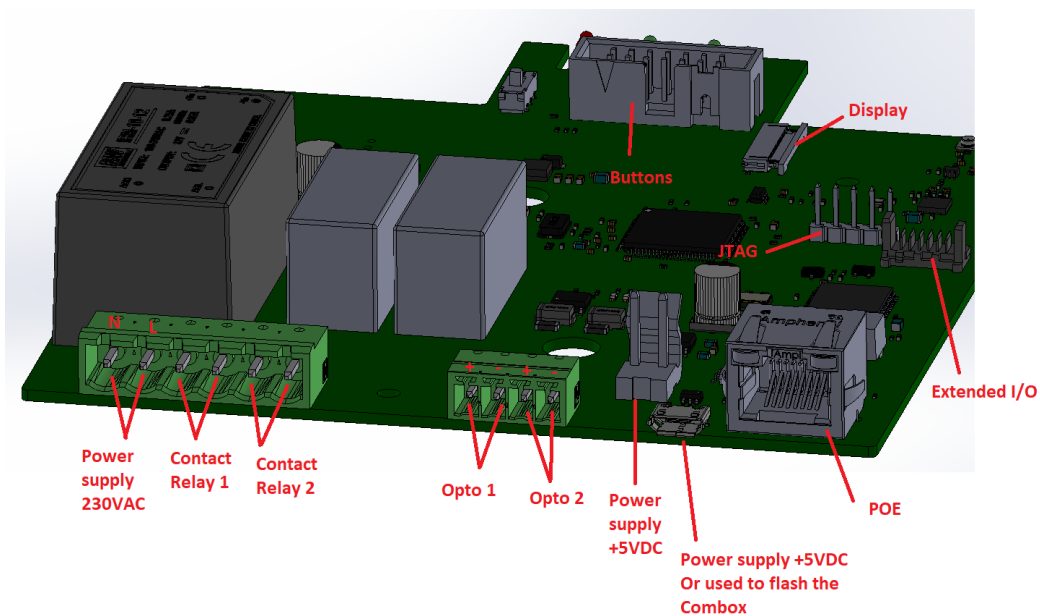
Illustration 12 : Motherboard connectors
