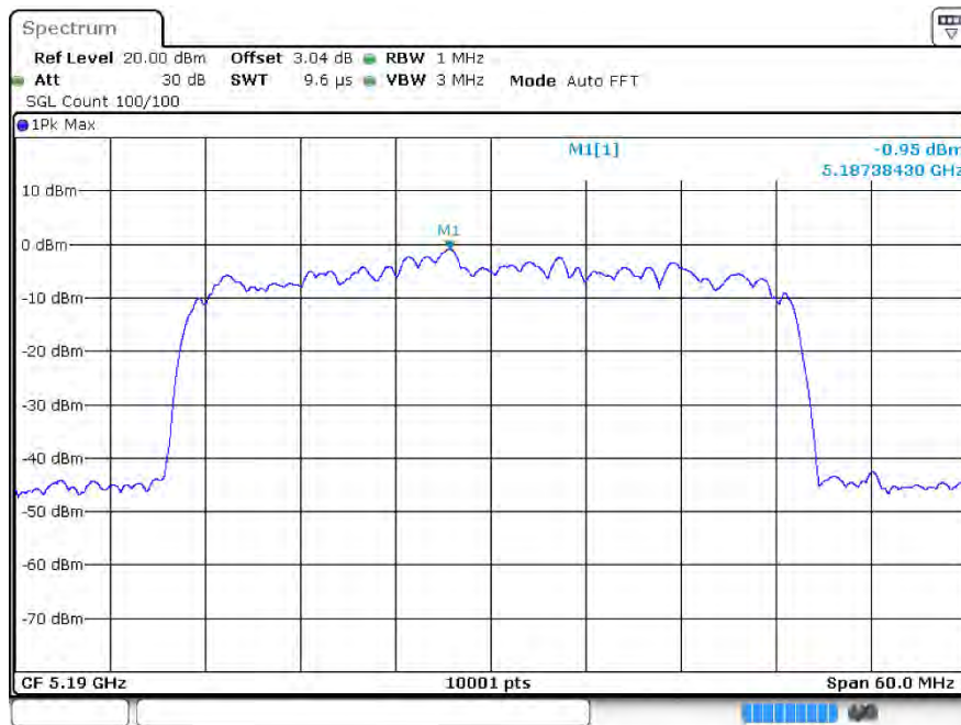
PSDax40 5190MHz Ant2
