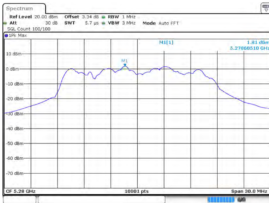
PSD ax20 5280MHz Ant2
