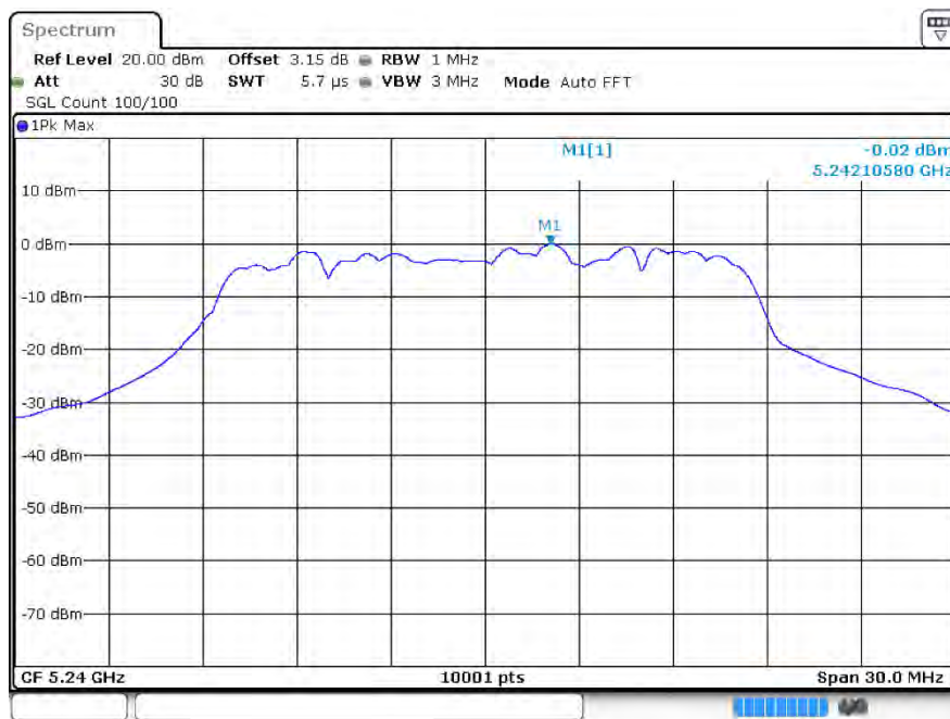
PSD ax20 5240MHz Ant2
