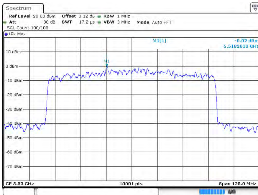
PSD ax80 5530MHz Ant2
