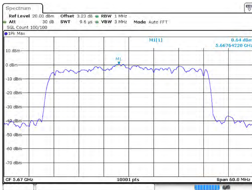
PSD ax40 5670MHz Ant2
