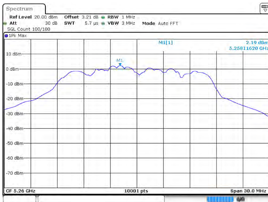
PSD ax20 5260MHz Ant2
