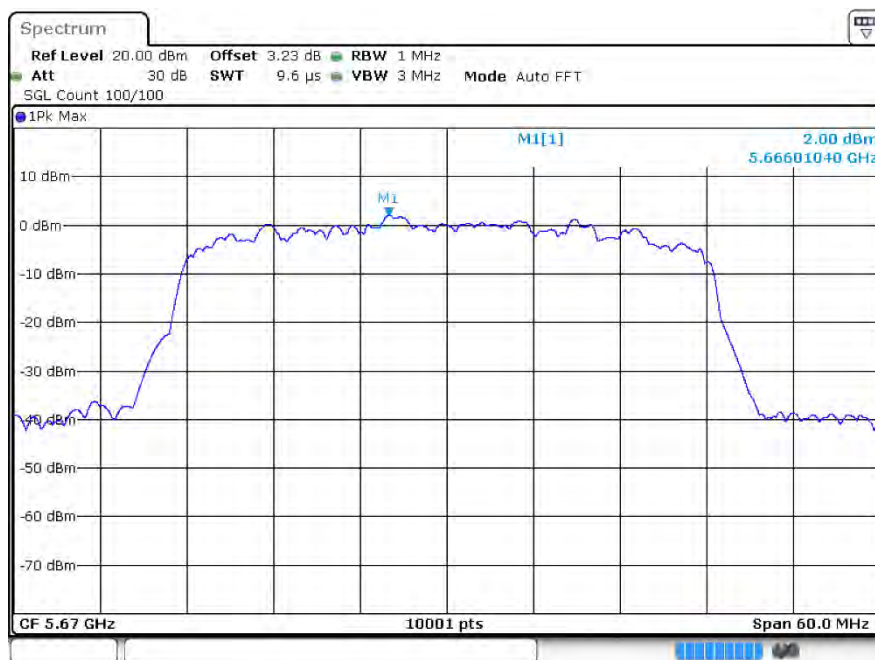
PSD ac40 5670MHz Ant2
