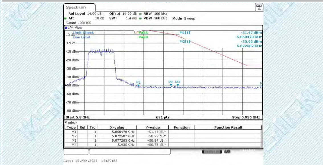
11N40SISO_Ant2_Low_5755
