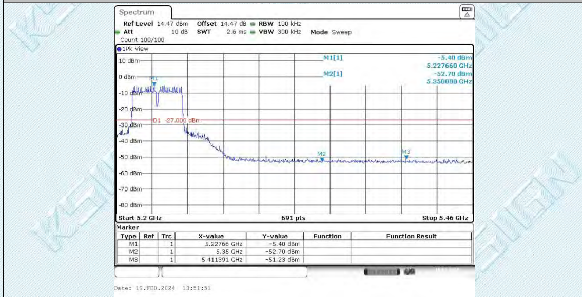
11AC80SISO_Ant2_Low_5210
