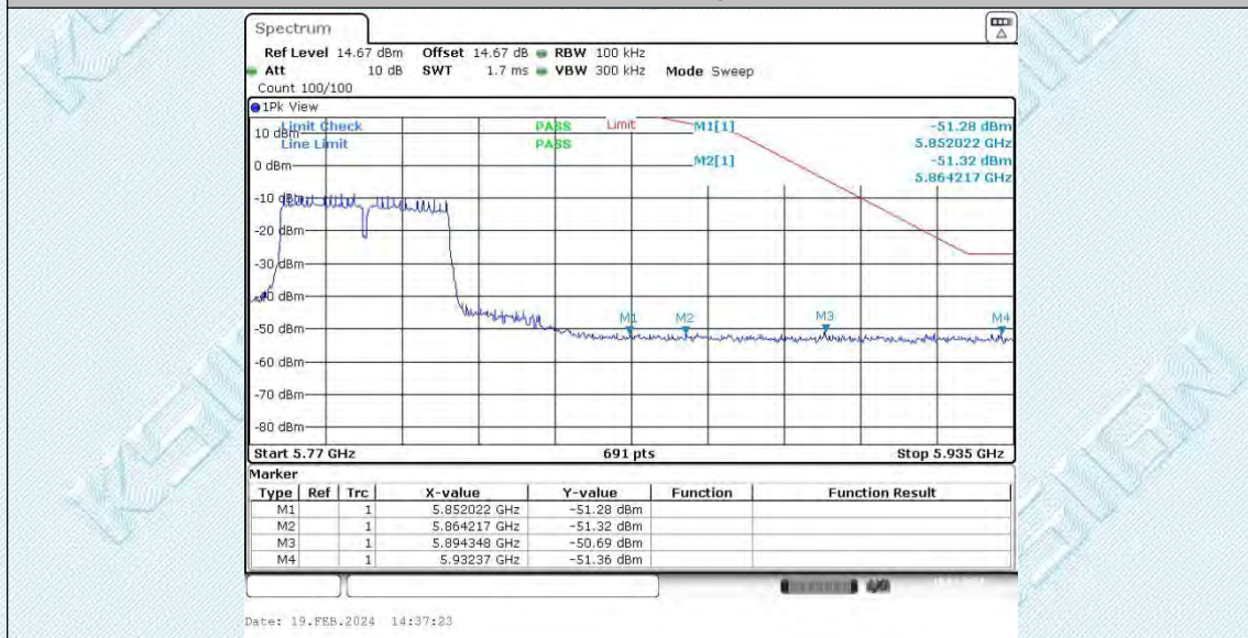
11AC80SISO_Ant2_Low_5775
