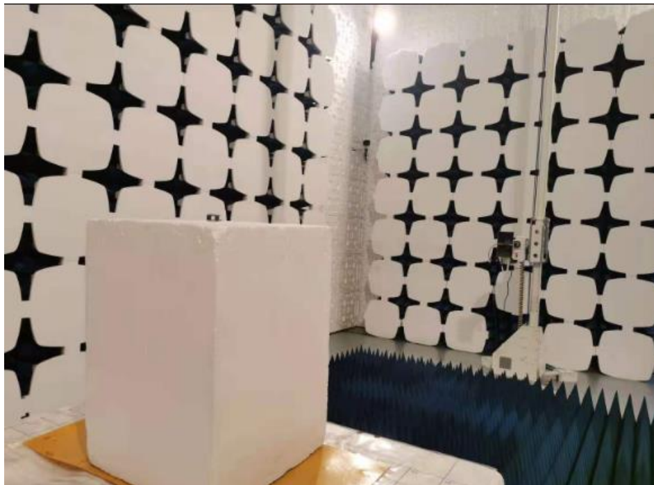
Above 1GHz
