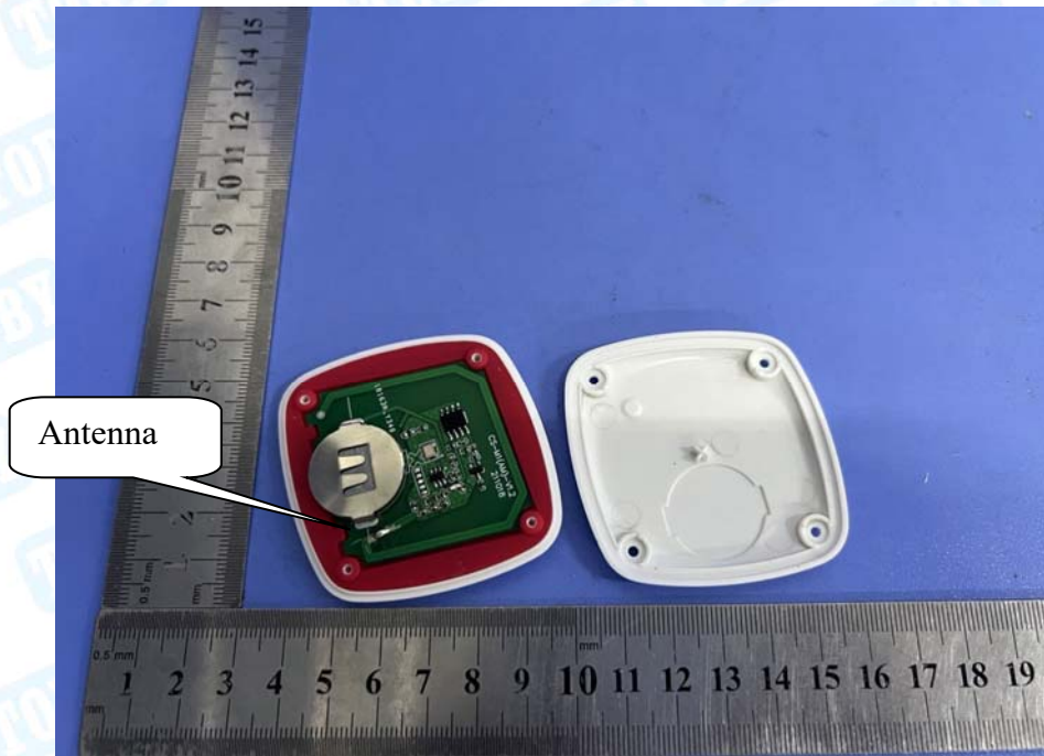
Photo 4 Internal of PCB
