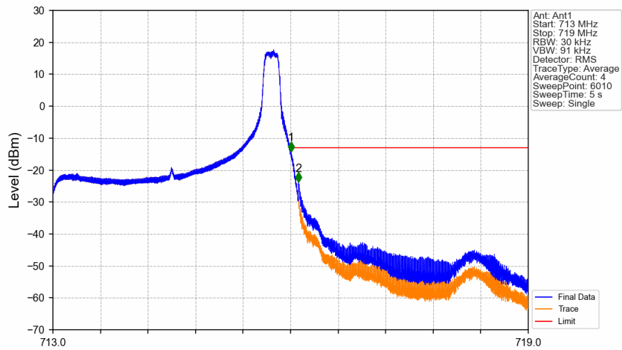
Band12_3MHz_QPSK_HCH_714.5MHz_RB_1_14_NTNV
