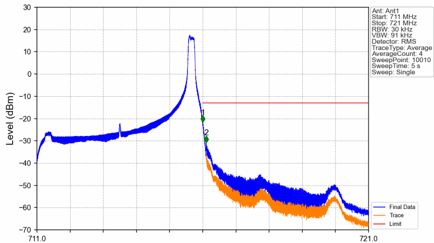
Band12_5MHz_QPSK_HCH_713.5MHz_RB_1_24_NTNV
