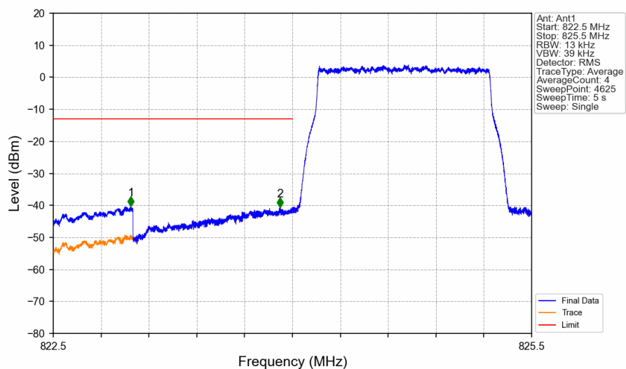
Band5 1.4MHz 16QAM LCH 824.7MHz RB 6 0 NTNV
