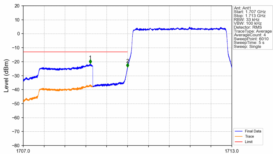
Band4_3MHz_QPSK_LCH_1711.5MHz_RB_15_0_NTNV
