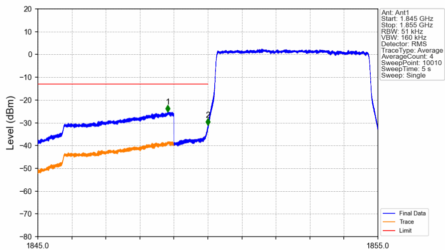
Band2_5MHz_QPSK_LCH_1852.5MHz_RB_25_0_NTNV
