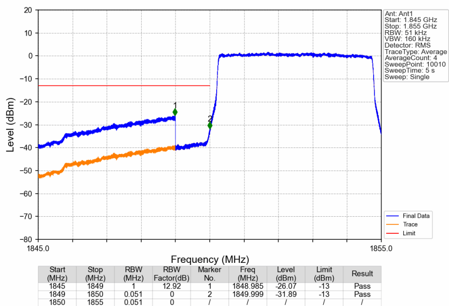
Band2_5MHz_16QAM_LCH_1852.5MHz_RB_25_0_NTNV
