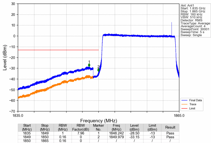
Band2_15MHz_16QAM_LCH_1857.5MHz_RB_75_0_NTNV
