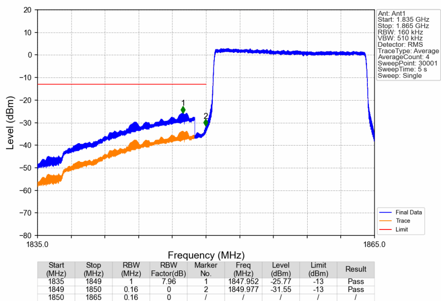
Band2_15MHz_QPSK_LCH_1857.5MHz_RB_75_0_NTNV
